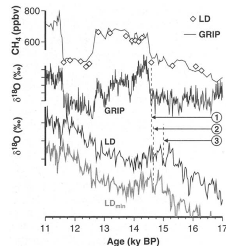
Fig. 2. Expanded view of the Law Dome isotope record under the two scenarios \text{LD}_{\text{min}} (minimum \Delta\text{age} chronology) and LD (default chronology) with GRIP \delta^{18}\text{O} and \text{CH}_4 [ \delta^{18}\text{O} scale unit 1 per mil (‰)]. Marker 1 (M1) indicates the timing of the last pre-Bølling \text{CH}_4 measurement. The northern Bølling transition cannot be placed earlier in time than M1. M2 and M3 show the ages of the enclosing ice for the gas sample at M1 under the two \Delta\text{age} scenarios. The intervals M2-M1 and M3-M1 are the \Delta\text{age} values for the \text{LD}_{\text{min}} and LD scenarios, respectively. Markers M2 and M3 on the isotope curves are located on, or around the peak marking the start of the ACR, which thus cannot be placed later in time than M1 ( \Delta\text{age} = 0 ). ppbv, parts per billion by volume.
