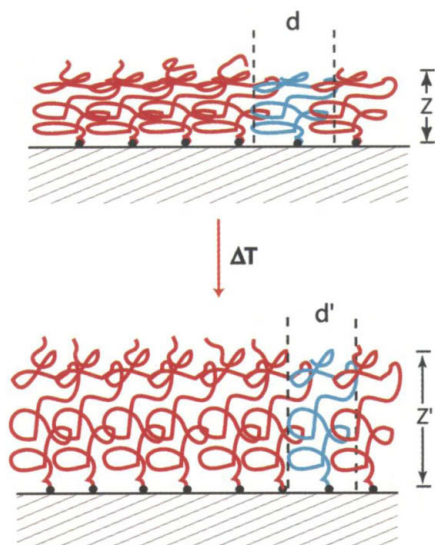
Fig. 2. Polymer chains anchored to a surface with a characteristic thickness Z and cross-sectional area A . Allowing the underlying substrate to relax causes the thickness to increase to Z' and the cross-sectional area to decrease to A' . The areal density of the chains has increased because of the relaxing of the underlying network. d and d' are the cross-sectional areas of the chains before and after contraction of the substrate by increasing the temperature by \Delta T .
