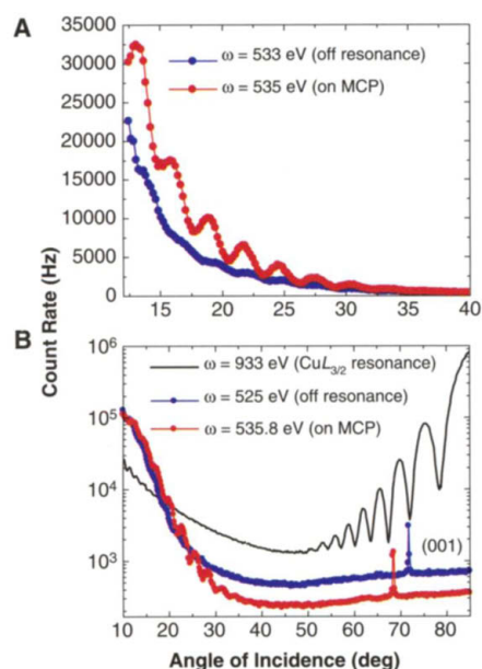
Fig. 3. Reflectivity of a 23.2-nm La 2 CuO 4+δ film ( T_c = 39 K) (A) just below and on the mobile carrier peak at 535 eV, showing the resonant enhancement; and (B) over the full angular range for three different energies. The 525-eV and 535.8-eV scans correspond to the reciprocal space interval (0,0,0.21) \rightarrow (0,0,1.21), whereas the 933-eV scan corresponds to (0,0,0.37) \rightarrow (0,0,2.15). The feature at 70° is the (001) Bragg reflection.
