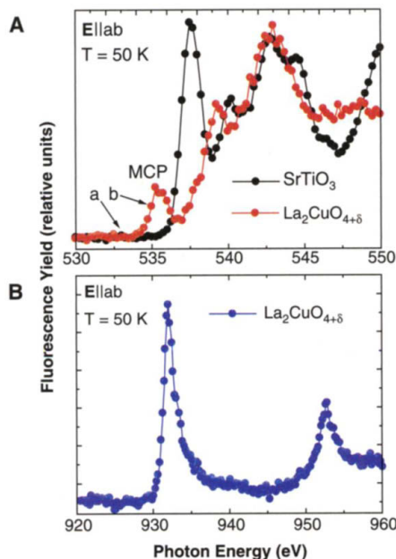
Fig. 1. X-ray absorption spectra of optimally doped \text{LaCuO}_{4+\delta} and \text{SrTiO}_3 , taken in fluorescence yield mode (A) in the vicinity of the \text{OK} edge, showing the mobile carrier peak set off from other features, and (B) at the \text{CuL} edge. All spectra are for \mathbf{E} \parallel \mathbf{ab} .
