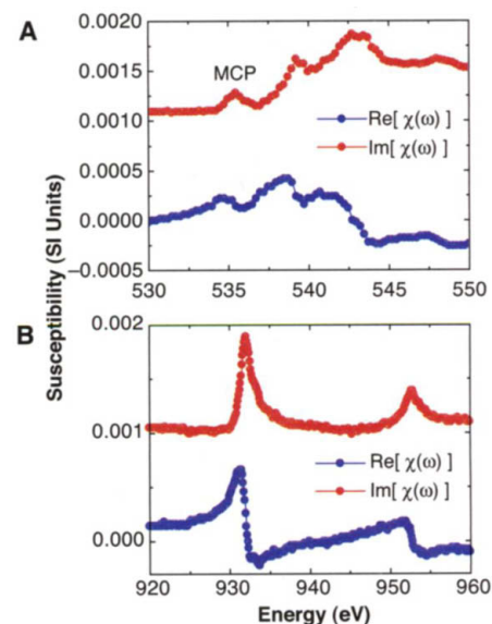
Fig. 2. ab -plane susceptibility of optimally doped \text{La}_2\text{CuO}_{4+\delta} , in SI units, calculated by the procedure described in the vicinity (A) of the \text{OK} edge and (B) of the \text{CuL}_{2,3} edge.
