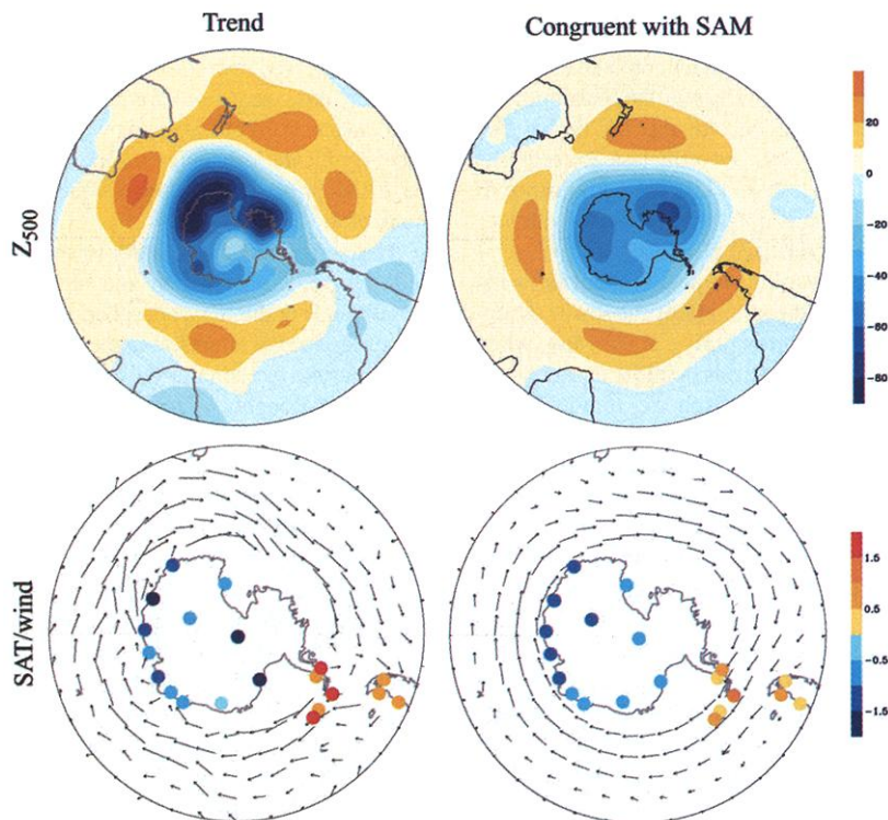
Fig. 3. December–May trends (left) and the contribution of the SAM to the trends (right). Top, 22-year (1979–2000) linear trends in 500-hPa geopotential height. Bottom: 32-year (1969–2000) linear trends in surface temperature and 22-year (1979–2000) linear trends in 925-hPa winds. Shading is drawn at 10 m per 30 years for 500-hPa height and at increments of 0.5 K per 30 years for surface temperature. The longest vector corresponds to ~4 m/s.
