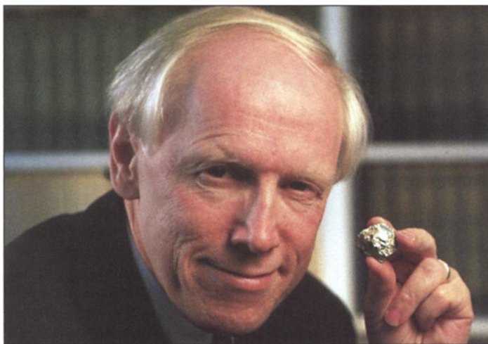
Molecular meeting place. Günter Wächtershäuser believes simple compounds necessary for life formed on lumps of pyrite.
