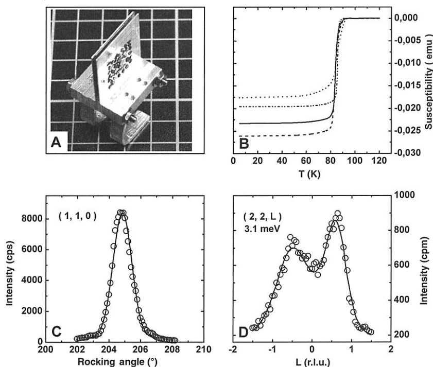
Fig. 1. (A) Photograph of the array of co-oriented \text{Ti}_2\text{Ba}_2\text{CuO}_{6+\delta} single crystals. The crystals are glued onto Al plates, only two of which are shown for clarity. (B) Typical diamagnetic shielding curves measured by superconducting quantum interference device (SQUID) magnetometry on individual crystals. (C) Rocking curve of the entire multicrystal array around the (1,1,0) Bragg reflection. The line is a Gaussian with a full width at half maximum of 1.5^\circ . (D) Constant-energy scan along \mathbf{Q} = (2,2,L) at excitation energy 3.1 meV and temperature 100 K, showing two counterpropagating transverse acoustic phonons. The wave vector \mathbf{Q} is given in reciprocal lattice units (r.l.u.). The data were taken at the 2T1 triple axis spectrometer at the Orphée research reactor (Saclay, France), with a pyrolytic graphite (PG) monochromator and a PG analyzer set at the (0,0,2) reflection and a fixed final energy of 14.7 meV. Three PG filters were inserted into the neutron beam to eliminate higher order contamination. The asymmetry of the profile is a resolution effect, and the solid line shows the result of a numerical convolution of a standard acoustic phonon dispersion with the spectrometer resolution. T, temperature; emu, electromagnetic units; cps, counts per second; cpm, counts per minute.
