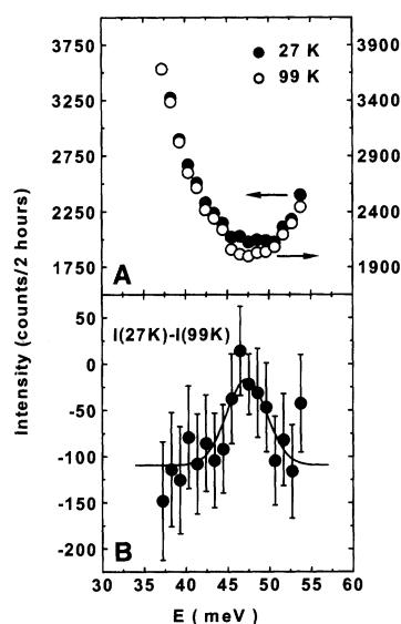
Fig. 3. Constant- Q scans at Q = (0.5, 0.5, 12.25) taken under the same conditions as the data of Fig. 1D. (A) Raw data at T = 99 K ( >T_c ) and T = 27 K ( <T_c ). (B) Difference between the two scans of (A). The line is a Gaussian profile whose width equals the experimental energy resolution.
