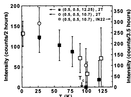
Fig. 4. Temperature dependence of the magnetic intensity extracted from fits to constant-energy scans at energy 47.5 meV around the in-plane wave vector Q_{AF} = \left(\frac{1}{2}, \frac{1}{2}\right) (Fig. 2).
