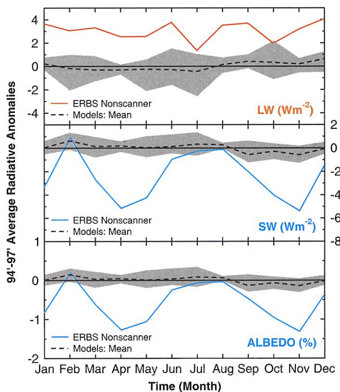
Fig. 4. Comparison of the observed broadband LW and SW flux anomalies for the tropics with climate model simulations using observed SST records. The models are not given volcanic aerosols, so they should not be expected to show the Mount Pinatubo eruption effects in mid-1991 through mid-1993. The dashed line shows the mean of all five models, and the gray band shows the total range of model anomalies (maximum to minimum).
