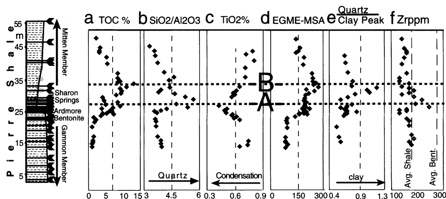
Fig. 2. Geochemical profiles [methods and data in (15)] of the Pierre Shale: (a) TOC; (b) \text{SiO}_2/\text{Al}_2\text{O}_3 (ratio of percentages), showing a maximum at horizon A likely corresponding to a decline in Al-rich detrital clay minerals (kaolinite) and an increase in aeolian quartz or biogenic silica; (c) \text{TiO}_2 minima, providing further evidence for condensation at horizon A implying a decline in detrital minerals, including silt-sized titanomagnetite, rutile, and sphene; (d) EGME-MSA for samples untreated with \text{H}_2\text{O}_2 ; (e) relative clay mineral versus quartz peak areas by XRD (clay minerals reach a maximum toward horizon B); (f) Zr used as an index of diagenetic smectite contribution from Zr-rich bentonite with global and average bentonite values from (10).
