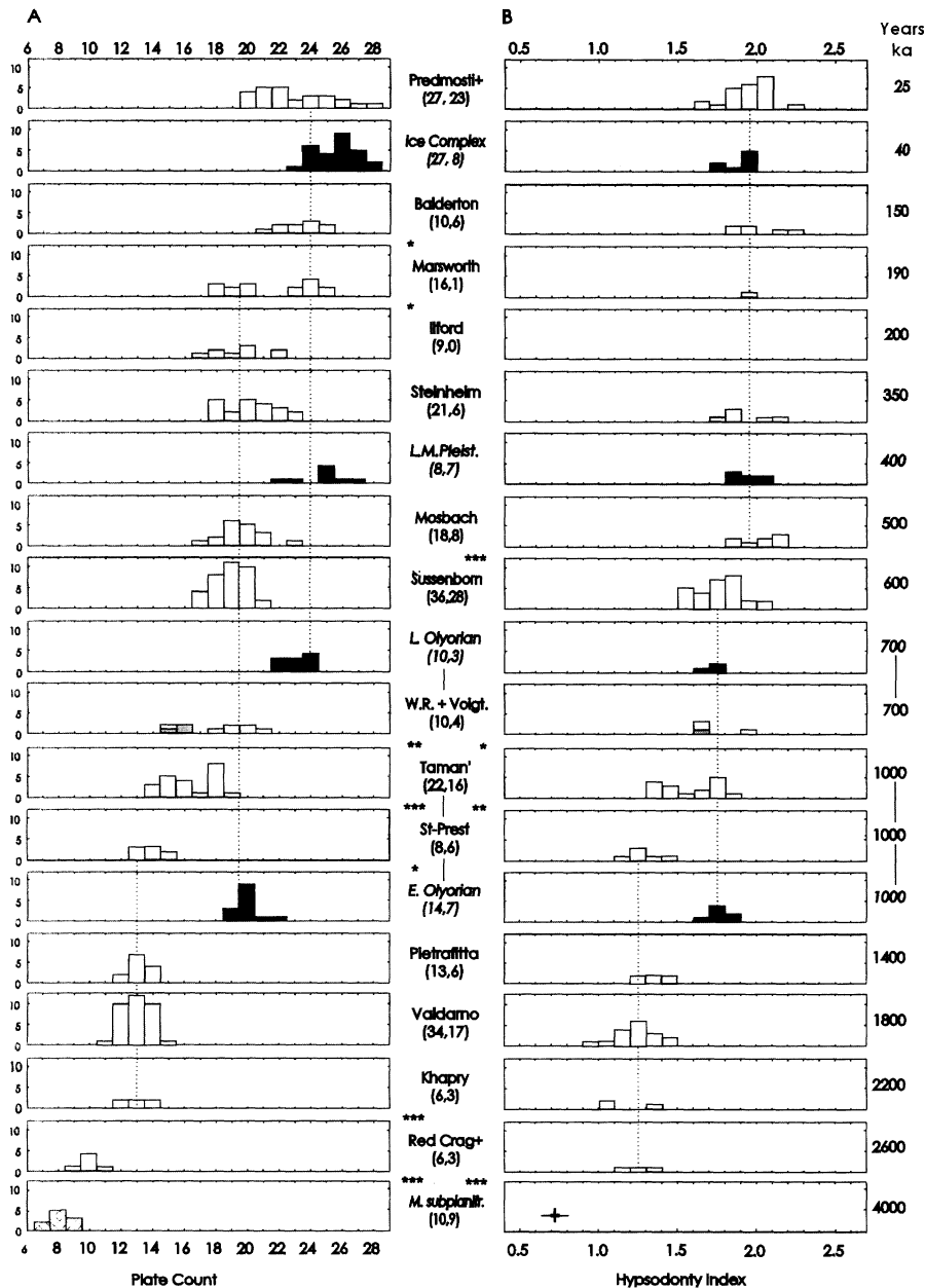
Fig. 3. (A) Plate count (P) of third upper plus lower molars; (B) hypsodonta index (HI) of third upper molars in the mammoth lineage. Open bars: European samples (shaded, Voigtstedt); filled bars and italic names/ages: northeastern Siberian samples; cross-hatched bars, African sample. Solid vertical lines connect sample names of equivalent age. Dotted lines traverse groups of samples (or subsamples, in the case of Taman' HI and West Runton and Marsworth P) at similar evolutionary level. Asterisks indicate conventional significance levels (two-tailed t tests; * P = 0.05, ** P = 0.01, *** P = 0.001) between successive, whole European samples only (i.e., bimodal samples are treated as a whole, and Siberian samples are ignored); P to the left of the central gutter, HI to the right. HI of M. subplanifrons is shown as mean \pm 1 standard error and 1 standard deviation, from (4). Sample sizes (P, HI) in brackets are after site names.
