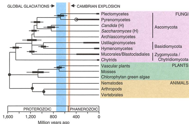
Fig. 3. Divergence time estimates for major groups of fungi, plants, and animals (Table 1). Thick horizontal bars on branch points are \pm 1 SE; narrow bars delimit 95% confidence intervals; thick bars on branches denote fossil record of fungi; solid circles are calibration points; open circle is internal (fungal) fossil constraint. H, Hemiascomycetes. The branching order of three groups (Ascomycota, Basidiomycota, Mucorales/Blastocladales) is shown as unresolved for topological consistency. On the basis of branching order from other data (11, 12), glomalean fungi diverged after chytrids and before the basidiomycotan/ascomycotan divergence, ~1400 to 1200 Ma.
