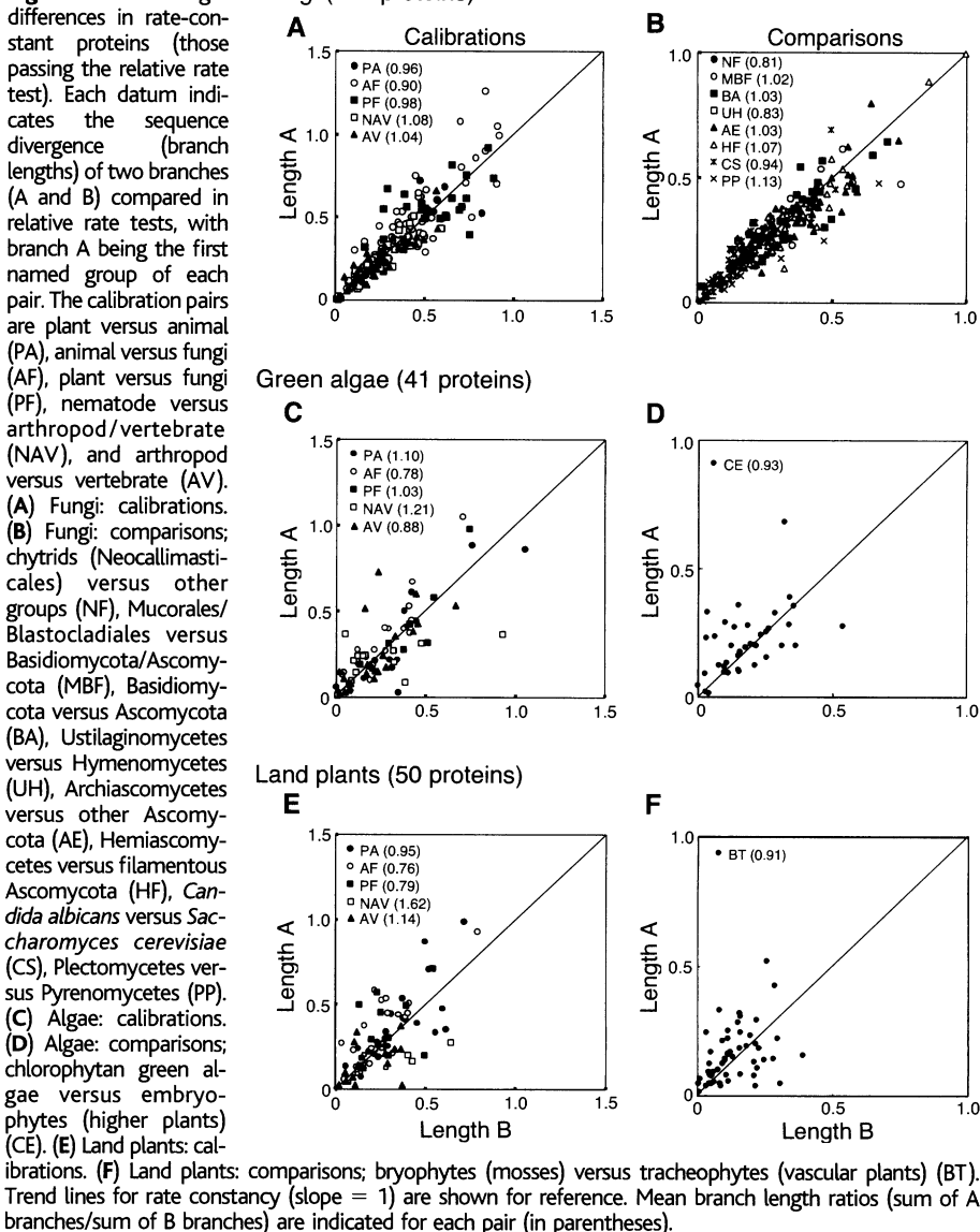
Fig. 1. Branch length differences in rate-constant proteins (those passing the relative rate test). Each datum indicates the sequence divergence (branch lengths) of two branches (A and B) compared in relative rate tests, with branch A being the first named group of each pair. The calibration pairs are plant versus animal (PA), animal versus fungi (AF), plant versus fungi (PF), nematode versus arthropod/vertebrate (NAV), and arthropod versus vertebrate (AV).
