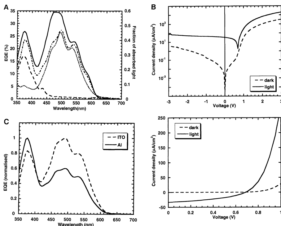
Fig. 4. (A) EQE action spectra for a 40:60 HBC-PhC 12 :perylene diimide blend (solid line) and the fraction of absorbed light in an HBC-PhC 12 film (dashed line), a perylene film (dotted line), and a 40:60 blend film (dash-dotted line). (B) Current-voltage characteristics for this device in the dark and under illumination at 490 nm. The short circuit current and open circuit voltage under illumination are -33.5 \mu\text{A}/\text{cm}^2 and 0.69 V, respectively, and the fill factor is 40%. The diode has a rectification ratio of 8.3 \times 10^2 at 2 V. (C) Normalized EQE action spectra taken under illumination through the ITO and Al electrodes, respectively, corrected for the absorption of the contacts and glass.
