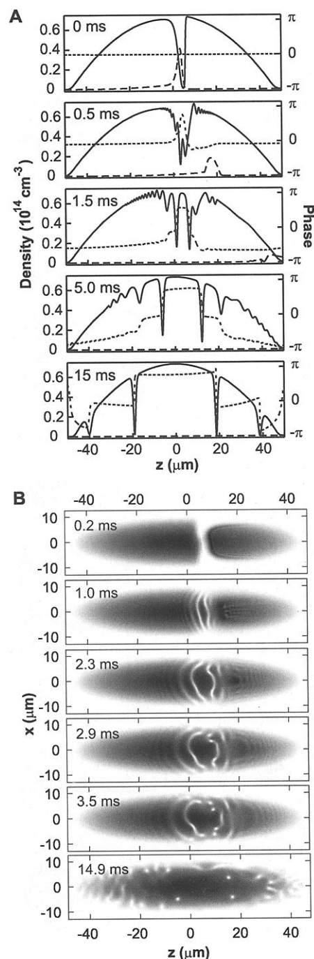
Fig. 3. (A) Formation of solitons from a density defect. The plots show results of a 1D numerical simulation of Eqs. 3 and 4. The light roadblock forms a defect, and the subsequent formation of solitons is seen. The defect is set up with the same parameters for the light fields as in Fig. 2B. The number of condensate atoms is N_c = 1.2 \times 10^6 and the peak density is 7.5 \times 10^{13} \text{ cm}^{-3} . The times in the plots indicate the evolution time relative to the time when the probe pulse stops at the roadblock and the coupling beam is switched off (at t = 8 \mu\text{s} , with t = 0 as defined in Fig. 1C). The solid and dashed curves show the densities of |1> atoms ( N_c|\psi_1|^2 ) and |2> atoms ( N_c|\psi_2|^2 ). The phase of \psi_1 is shown in each case with a dotted curve (with an arbitrary constant added for graphical clarity). In the first two frames, the |2> atoms quickly leave as a result of the momentum recoil, leaving a large-amplitude, narrow defect in \psi_1 (because this is a 1D simulation, the momentum kick in the x direction is ignored). (B) The snake instability and the nucleation of vortices. The plots show the density N_c|\psi_1|^2 from a numerical simulation in 2D, with white corresponding to zero density and black to the peak density ( 6.9 \times 10^{13} \text{ cm}^{-3} ). The parameters are the same as in Fig. 2B, and the times indicated are relative to the coupling beam turnoff at t = 21 \mu\text{s} . The solitons curl about their deepest point, eventually breaking and forming vortex pairs of opposite circulation (seen first at 3.5 ms). Several vortices are formed, and the last frame shows the vortices slowly moving toward the edge of the condensate. At later times, they interact with sound waves that have reflected off the condensate boundaries. Animated versions are provided in (40).
