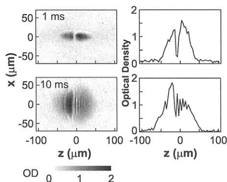
Fig. 4. Experimental OD images and line cuts (at x = 0 ) of a localized defect (top) and the resulting formation of solitons (bottom) in a condensate of |1\rangle atoms. The imaging beam was detuned -30\ \text{MHz} and -20\ \text{MHz} , respectively, from the |3S_{1/2}, F = 2\rangle \rightarrow |3P_{3/2}, F = 3\rangle transition. Before imaging, the atoms were optically pumped to |3S_{1/2}, F = 2\rangle for 10\ \mu\text{s} . The probe pulse had a peak Rabi frequency \Omega_p = (2\pi)2.4\ \text{MHz} . The coupling laser had a Rabi frequency \Omega_c = (2\pi)14.9\ \text{MHz} , was turned on 6\ \mu\text{s} before the probe pulse maximum, and had a duration of 18\ \mu\text{s} .
