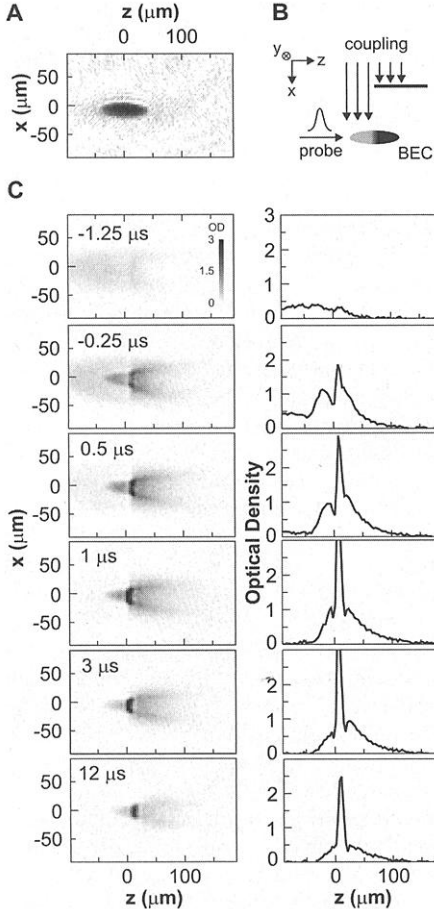
Fig. 1. (A) Experimental in-trap OD image of a typical BEC before illumination by the probe pulse and coupling field. The condensate contains 1.5 \times 10^6 atoms. The imaging beam was -30 \text{ MHz} detuned from the |1\rangle \rightarrow |3P_{1/2}, F=2, M_F=-1\rangle transition. (B) Top view of the beam configuration used to create and study localized defects in a BEC. (C) Buildup of state |2\rangle atoms at the roadblock. In-trap OD images (left) show the transfer of atoms from |1\rangle to |2\rangle as the probe pulse propagates through the condensate and runs into the roadblock. The atoms in |2\rangle were imaged with a laser beam -13 \text{ MHz} detuned from the |2\rangle \rightarrow |3P_{3/2}, F=3, M_F=-2\rangle transition. To allow imaging, we stopped the probe pulse propagation at the indicated times by switching the coupling beam off (29). The time origin t = 0 is defined as the moment when the center of the probe pulse enters the BEC from the left. The graphs on the right show the corresponding line cuts along the probe propagation direction through the center of the BEC. The probe pulse had a Rabi frequency \Omega_p = (2\pi)2.4 \text{ MHz} , and the coupling Rabi frequency was \Omega_c = (2\pi)14.6 \text{ MHz} .
