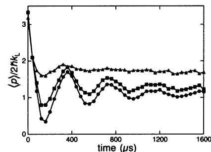
Fig. 2. Comparison of tunneling oscillations for different Raman detunings. The strongest oscillations observed (●) correspond to Raman velocity selection at p = 0 . The other two cases are for velocity selection at p = 0.05 \times 2\hbar k_L (■), where the oscillations are partially suppressed, and p = 0.12 \times 2\hbar k_L (▲), where the oscillations are almost completely suppressed.
