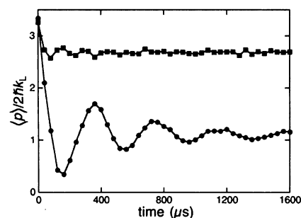
Fig. 4. Comparison of chaos-assisted tunneling oscillations (●) to transport in the corresponding quantum pendulum (■). No tunneling oscillations are observed in the pendulum case over the interaction times studied in the experiment.
