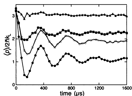
Fig. 3. Comparison of chaos-assisted tunneling for different free-drift times before the standing-wave interaction. The strongest oscillations occur for zero drift time (●), where the initial wave packet is centered on the island of stability as in Fig. 1A. The oscillations are substantially suppressed for a 3.8- \mu s drift time (■), which displaces the initial wave packet center by 1/4 of a period of the standing wave. Tunneling oscillations are completely suppressed for a 7.6- \mu s drift time (▲), corresponding to a 1/2 -period offset of the initial wave packet. For a 15.1- \mu s drift time (○), the wave packet is again centered on the island, and coherent oscillations are restored.
