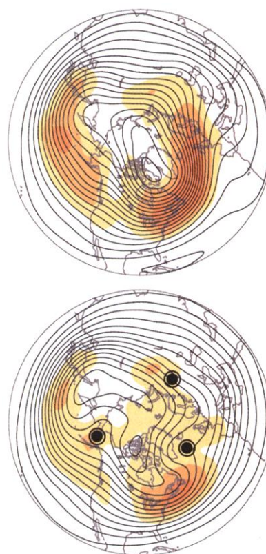
Fig. 3. As in Fig. 2, but for composite maps of 500-hPa height (contours) and the SD of band-pass filtered 500-hPa height field (shading) (18). Blocking regions (14) used in Table 2 are marked by black dots. Contour intervals are 50 m for 500-hPa height (the lowest contour is 4950 m in the high-index composite and 5150 m in the low-index composite). Shading is drawn for SD values of 50, 60, and 70 m.
