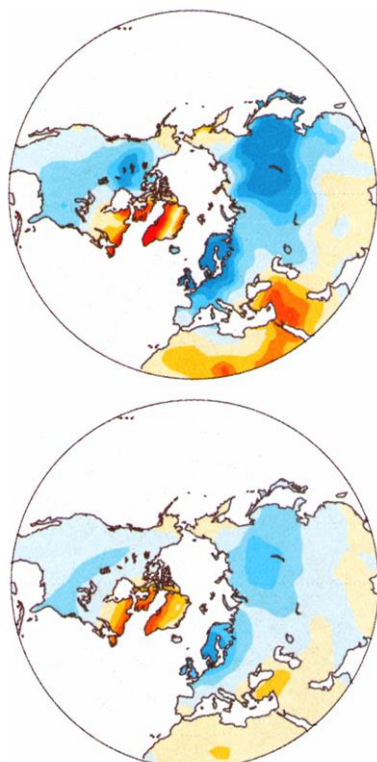
Fig. 4. The signature of the NAM in the frequency of occurrence of cold events (daily minimum temperature <1.5 SD below the climatological mean) based on 6-hourly JFM data, 1958–1997, from the NCEP/NCAR Reanalysis (10). (Top) The ratios of the number of cold events in the low NAM-index sample to the number of cold events in the high NAM-index sample. (Bottom) As in the top panel, but for the ratios attributable to shifts in mean temperature (19). Shading is drawn for ratios \pm 2:1 , 3:1 , 4:1 , and 6:1 . Blue shading indicates more cold events under low index conditions. Ratios > 2:1 exceed the 95% confidence level (15).
