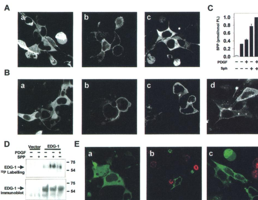
Fig. 3. SPP produced intracellularly can act in an autocrine or paracrine fashion to activate EDG-1. (A) \beta -Arrestin translocation in HEK 293 cells cotransfected with expression plasmids encoding \beta -arrestin2-GFP and EDG-1. \beta -Arrestin2-GFP fluorescence was visualized (10) after treatment with vehicle (a), 100 nM SPP (b), or 5 \mu M sphingosine (c). (B) Translocation of \beta -arrestin in HEK 293 cells cotransfected with \beta -arrestin2-GFP, EDG-1, and SPHK1. \beta -Arrestin2-GFP fluorescence was visualized after treatment with vehicle (a), 100 nM SPP (b), 2.5 \mu M sphingosine and 20 ng/ml PDGF-BB (c), or 5 \mu M sphingosine (d). (C) Cellular levels of SPP. Levels of SPP were measured in vector-transfected (white bar) and in SPHK1-transfected (filled bars) HEK 293 cells after treatment with 2.5 \mu M sphingosine, 20 ng/ml PDGF-BB, or both for 10 min (20). (D) PDGF-induced EDG-1 phosphorylation. Vector or Flag-EDG-1-expressing HEK 293 cells were transfected with PDGFR- \beta and cultured in 10% charcoal-stripped FBS for 24 hours, metabolically labeled in phosphate-free Dulbecco's modified Eagle's medium with [ ^{32} P]orthophosphate (70 \mu Ci/ml) for 2.5 hours at 37°C, then stimulated with SPP (100 nM) or PDGF (20 ng/ml). Cell lysates were prepared and immunoprecipitated with antibody against Flag M2 (Sigma) as described (15). Immunoprecipitates were either separated on 10% SDS-PAGE, transblotted to nitrocellulose, and autoradiographed (upper panel) or immunoblotted with antibody against Flag (lower panel). (E) \beta -Arrestin translocation in HEK 293 cells cotransfected with \beta -arrestin2-GFP, EDG-1, and empty vector for SPHK1 (green cells). Conditioned medium from \beta -arrestin2-RFP, EDG-1, and SPHK1 transfectants (red cells) that had been treated with 5 \mu M sphingosine to generate intracellular SPP (a) or the cells themselves (b and c) were added to "green" cells. \beta -Arrestin2-GFP and \beta -arrestin2-RFP fluorescence was visualized by using dual excitation (488 and 568 nm) and emission (515 to 540 nm, GFP; 590 to 610 nm, RFP) filter sets (10).
