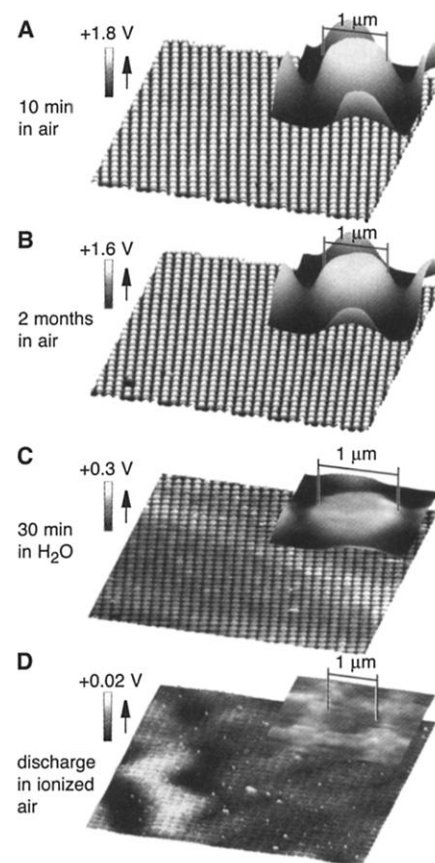
Fig. 3. Stability of the patterned charge in air, water, and ionized air. Surface potential distribution recorded (A) immediately after formation and (B) after 2 months aging in air. (C) Surface potential distribution upon exposing the charge pattern to deionized water. (D) Surface potential distribution upon discharge with ionized air.
