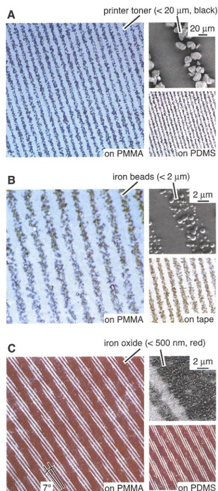
Fig. 5. Optical microscope and SEM images of different types of particles trapped at patterned charge and transferred onto second substrates. (A) 50- \mu m-wide parallel lines of toner particles, <20 \mu m in size; (B) 5- \mu m-wide parallel lines of iron beads, <2 \mu m in size; (C) 2.5- and 10- \mu m-wide lines of red iron oxide particles, <500 nm in size, crossing at 7° incidence. In this demonstration, all particles were trapped with positive charge that was patterned with stamps carrying parallel lines 2.5, 5, and 10 \mu m wide. The crossing lines were fabricated by two exposures at different angles. The insets labeled "on tape" and "on PDMS" are images of patterns of particles transferred to Scotch tape and PDMS, respectively, by contact. All optical images are in true color. Contrast and brightness have been adjusted slightly.
