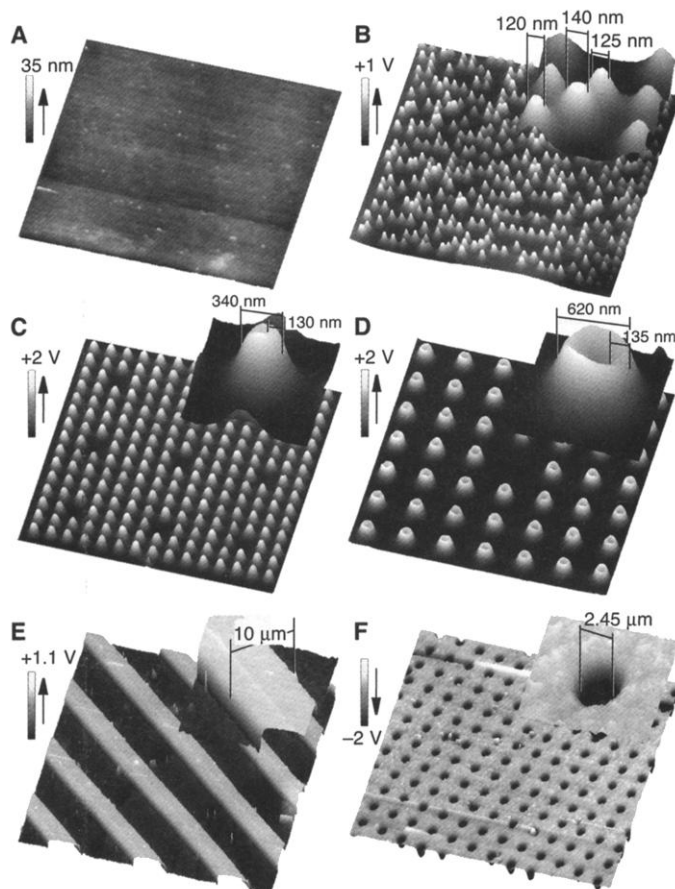
Fig. 2. KFM images of patterns of positive and negative surface potential generated by e- \mu CP. (A) Surface topography and (B) surface potential distribution of a test pattern of high-density data storage with <150\text{-nm} -sized bits (FWHM). The pattern was generated using a stamp carrying 150\text{-nm} -wide circular posts that were 90\text{ nm} high. (C and D) Surface potential images of ring-type charge patterns generated using a stamp carrying 350\text{-} and 640\text{-nm} -wide circular posts that were slightly higher at the edge than in the center. (E) Surface potential image of positively charged parallel lines generated using a stamp carrying 10\text{-}\mu\text{m} -wide parallel lines that were 850\text{ nm} high. (F) Surface potential images of negatively charged dots generated using a stamp carrying 2.5\text{-}\mu\text{m} -wide circular posts that were 850\text{ nm} high. The amplitudes of the surface potentials in these figures cannot be compared directly.
