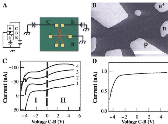
Fig. 2. Shown are n + - p - n SiNW bipolar transistors. (A) Schematics illustrating the common base configuration of an n + - p - n bipolar transistor (19) and the corresponding structure built from crossed SiNWs (right). The n + -, p -, and n -type SiNWs function as emitter, base, and collector, respectively. (B) Typical FESEM image of SiNW bipolar transistor. The three wires labeled as n + , p , and n were used as emitter, base, and collector, respectively. Scale bar, 5 \mu m. (C) Collector current versus collector-base voltage recorded on an n + - p - n transistor with emitter and collector SiNWs 15 \mu m apart. Curves 1 to 4 correspond to the data recorded for emitter-base voltages of -1, -2, -3, -4 V, respectively. Regime I and II are separated by a dashed line, corresponding to saturation mode and active mode, respectively. (D), The common base current gain versus collector-base voltage.
