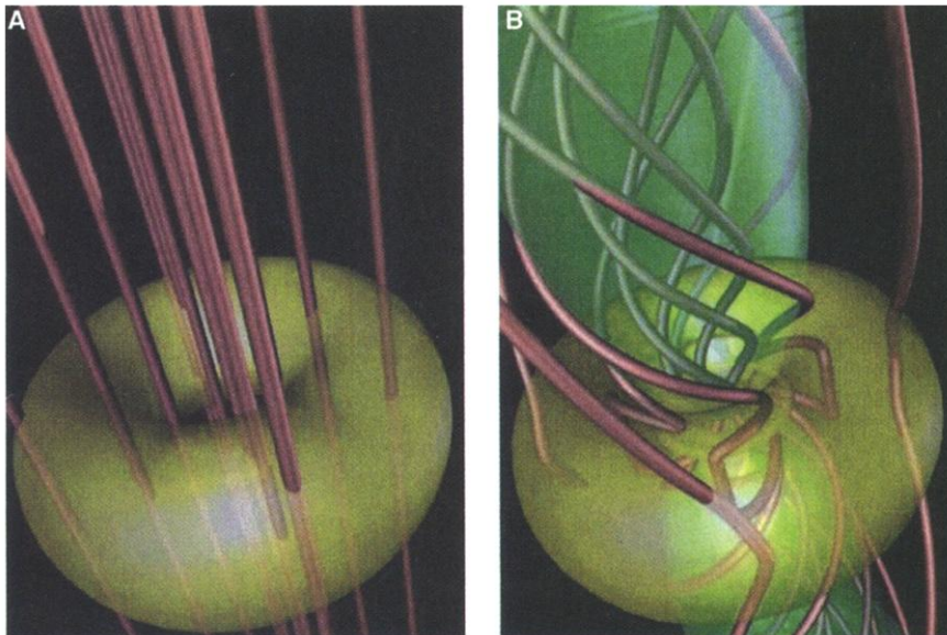
Fig. 5. An MHD simulation of a thick magnetized torus surrounding a supermassive ( 10^8 M_\odot ) central object (26). (A) Initial state showing the torus in rotational equilibrium with an axial magnetic field. (B) As the simulation begins, the differentially rotating torus drags the field lines in the azimuthal direction, creating a braking force that allows the material to accrete inward and gain additional rotational energy. The effect of this process is to produce a torque on the external magnetic field, generating a torsional Alfvén wave and a spinning plasma jet that carries away matter, angular momentum, and energy from the system. Far above the disk, the torsional waves will be unstable to the helical-kink instability, generating the wiggled structure seen in Fig. 2.
