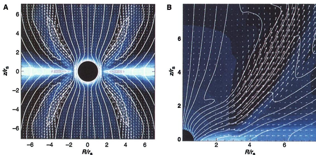
Fig. 6. Two fully general relativistic simulations of jet production by accretion disks around black holes. Each begins with an axial field. Plots are meridional cuts, with length units in Schwarzschild radii ( 2R_g ), and show the plasma density in blue-white color, poloidal velocity vectors with white arrows, and a poloidal magnetic field as solid white lines. (A) A nonrotating, Schwarzschild hole with a moderately strongly magnetized Keplerian disk whose rotation drives an MHD jet at the escape speed ( \sim 0.4c ) [from (28)]. (In this simulation, a gas-pressure-driven outflow also is ejected from a radius interior to the last stable orbit at a somewhat higher speed.) (B) A rotating Kerr hole ( j = 0.95 ) (in the lower left corner) with a nonrotating disk [from (30)]. Preliminary analysis indicates that the dragging of inertial frames drives the jet from a region just outside the ergosphere at R \sim 1r_s to 2r_s ( 2R_g to 4R_g ) at the escape speed of \sim 0.93c ( \Gamma \approx 2.7 ).
