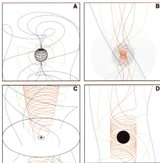
Fig. 4. Schematic diagrams of four astrophysical scenarios in which differential rotation of a magnetic field might generate relativistic jet outflow. Color is used to aid in identification of the field lines. (A) The dipole field of a heavily accreting, rapidly rotating pulsar can be swept back by the accreting matter as close as a few tens of kilometers from the stellar surface. Some of this material will be ejected in a jet at the local escape speed. (B) A slowly rotating pre-supernova white dwarf or dense stellar core will collapse to a rapidly rotating proto-neutron star. Even an initially uniform axial field will be drawn inward and wound into a tight coil, ejecting some of the dense core material. The jet may have sufficient power to alter the shape of the supernova ejecta or even drive the explosion on its own. (C) The poloidal magnetic field protruding from an accretion disk orbiting a compact object will fling disk coronal material outward in a wind. Conservation of angular momentum will slow the wind's rotation and, if the outflow is dense enough, sweep back and coil the field lines. (D) Near a rotating black hole, the space itself rotates differentially. This dragging of inertial frames is particularly strong inside a radius about twice that of the hole—the ergosphere—where material must rotate with the hole. Here only the twisting of vertical field lines is shown, but as the plasma accretes toward the black hole, these lines will be drawn inward, creating a structure similar to that in (B) or (C).
