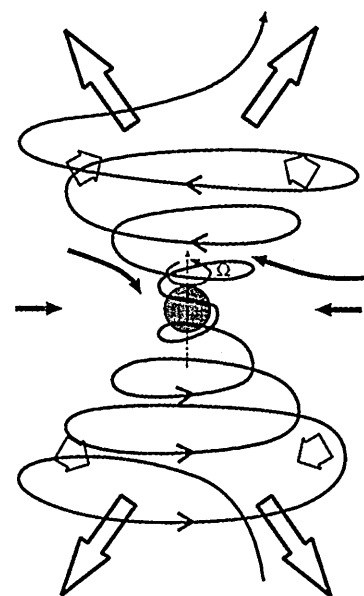
Fig. 3. Schematic diagram depicting the MHD acceleration and collimation model. Magnetized and rotating inflow toward a compact object (solid arrows) winds the magnetic field lines into a rotating helical coil called a torsional Alfvén wave train (TAWT). Magnetocentrifugal forces expel some of the material along the field lines and magnetic pressure and pinching forces (short open arrows) further lift and collimate it into a jet outflow (long open arrows).
