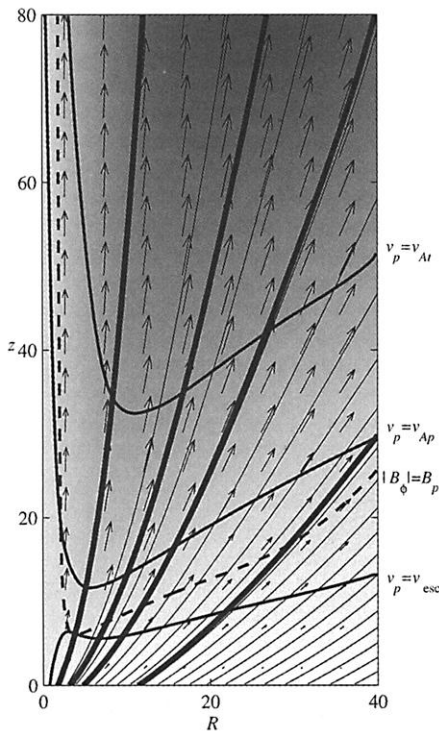
Fig. 7. An accretion disk wind in a steady state [from (34) and similar to results in (33)]. The central object is at (0, 0), and the infinitely thin disk is along Z = 0 . Arrows indicate velocity vectors. Lines anchored in the disk and arching upward are contours of magnetic flux; the dashed curve indicates the surface above which the strength of the azimuthal ( B_\phi ) component of the twisting magnetic field exceeds the poloidal field strength [ B_p = (B_r^2 + B_z^2)^{1/2} ]; and the three labeled curves show surfaces where the poloidal velocity achieves the escape velocity, the poloidal Alfvén velocity (determined by the poloidal field alone), and the total Alfvén velocity. Any transient properties of the flow have disappeared, leaving a slowly accelerating bipolar wind that collimates from opening angles of \sim 40^\circ to 50^\circ to only a few degrees over many tens of inner disk radii. Such a picture is qualitatively and, perhaps, quantitatively similar to the wide opening angles observed in M87 in the inner core (Fig. 1). [Figure courtesy of R. Krasnopolsky]
