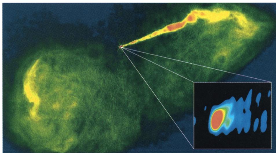
Fig. 1. The jet in the galaxy M87 displays most of the important features of relativistic jets. The approaching northwest jet is Doppler boosted, whereas the southeast one is virtually undetectable because it radiates away from Earth. The lobes, consisting of decelerated jet material, radiate isotropically, and therefore both are visible. The full extent of the source projected on the sky in this image is \sim 80 arc sec or 6 kpc. Because the source is at an angle of < 19^\circ to our line of sight, its deprojected length must be at least 20 kpc. Deep in the core (inset), the jet shows an initial wide opening angle ( 60^\circ ) that decreases with distance from the core. This indicates that the acceleration and collimation region may be resolved. The length of the jet emission in the inset is \sim 0.001 arc sec or 16,000 astronomical units, which is only \sim 250 times the Schwarzschild radius of the central 3 \times 10^9 M_\odot black hole. [Images were made with the National Radio Astronomy Observatory's Very Large Array and Very Long Baseline Array and are courtesy of J. Biretta and W. Junor; reprinted by permission from Nature (37) copyright (1999) Macmillan Magazines Ltd.]
