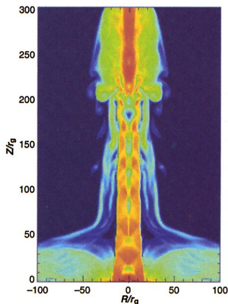
Fig. 8. Illustration of an efficient high MHD power jet, with L_{\text{MHD}} = 1.5 L_{\text{crit}} [from (54)]. The diagram shows the strength of the magnetic pressure ( B^2/8\pi ) at a model time of \sim 10 inner disk rotation times, with red indicating the strongest pressure and blue indicating the weakest. Acceleration occurs much faster than the dynamical rate. The flow reaches a quasi-steady state quickly, with a tightly collimated jet above the escape speed. Although more powerful, the jet delivers its thrust in a narrow solid angle, affecting the surrounding ambient material much less than the slower, broad outflow in Fig. 7.
