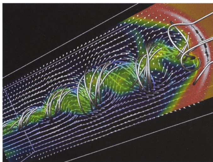
Fig. 2. A three-dimensional simulation of the propagation of a magnetized jet, which depicts most of the properties of the MHD model. The diagram shows flow velocity (arrows), the plasma density field (color, with white and blue indicating high and low pressure, respectively), and the magnetic lines of force (metallic tubes). The initially axisymmetric, rotating jet has developed a helical-kink instability that distorts its shape. The plasma flow still follows the field lines. Such an instability may explain the wiggles observed in some parsec-scale radio jets. The super-Alfvénic jet terminates in a strong shock wave at right, as it propagates into a region with decreasing Alfvén velocity. High-energy particles accelerated in the rotating magnetic twists, and especially in the compressed field behind the bow shock, will emit synchrotron radiation. This shock therefore may correspond to the hot spot often seen at the end of jets in many radio sources. [Courtesy of M. Nakamura]
