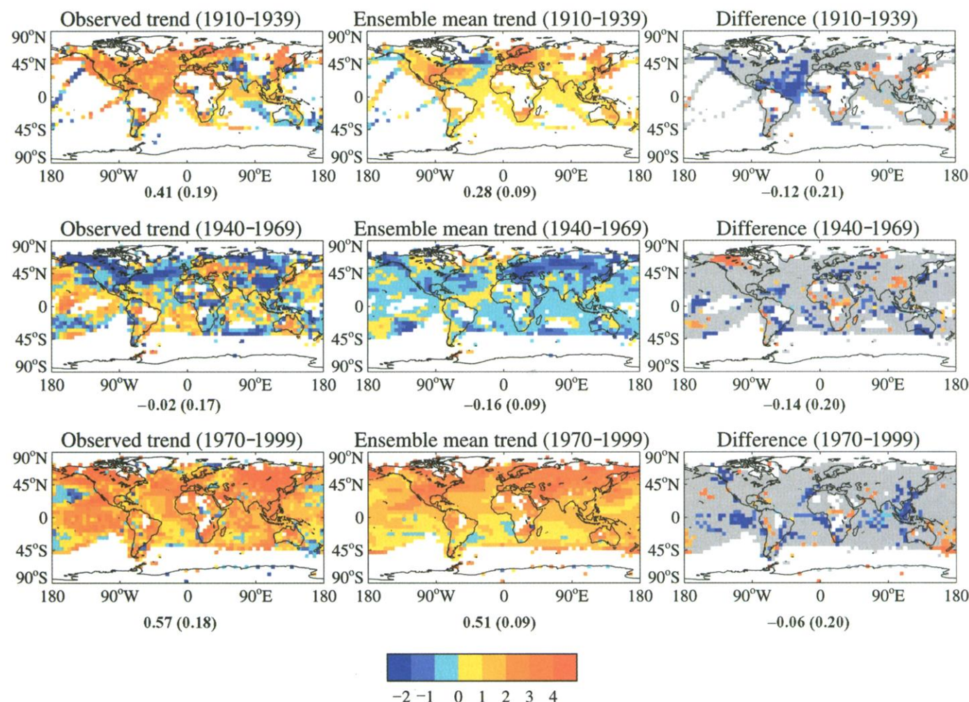
Fig. 3. Linear trends (K/30 years) of near-surface temperature for three 30-year periods spanning 1910 to 1999 from the observations, the ALL ensemble mean, and model-observational differences significant at the P = 0.10 level according to a two-sided t test. Gray shading denotes regions
