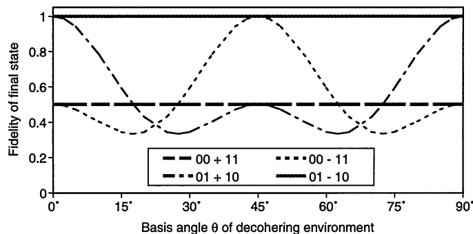
Fig. 1. Theoretically calculated fidelity of final state with initial Bell state, after collective decoherence in the (linear-polarization) basis \theta/\theta^\pm . The fidelity between any Bell state and a completely mixed state is 0.25; the minimum predicted fidelities are 0.33.
