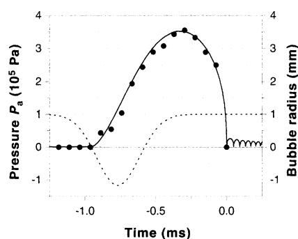
Fig. 3. The calculated bubble radius R(t) as a function of time (solid line). The temporal change of the pressure field P(t) that was modeled for this calculation is also given (dashed line). The model parameters ( P_a = 2.2 \times 10^5 Pa and \sigma = 360 \mu s) were fitted to match the theoretical radius with the experimentally determined equivalent bubble radius of the ellipsoidal cavitation bubble (indicated by solid circles).
