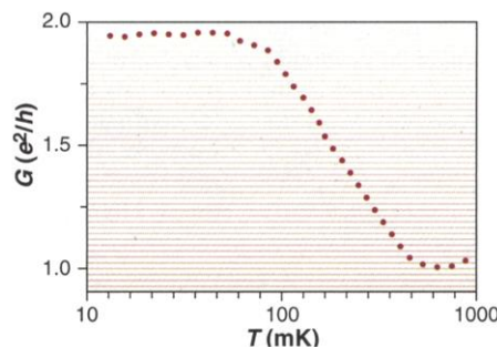
Toward the unitary limit. Temperature dependence of the height of the peak in G(V) , which saturates near the unitarity limit of 2e^2/h for van der Wiel et al. 's QD.
