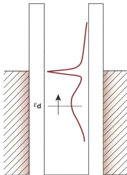
Effective screening. Energy diagram for a QD whose density of states (dashed line) has a broad single-particle resonance at the energy of the local level, \epsilon_d , and a sharp Kondo resonance at the chemical potential of the leads.
