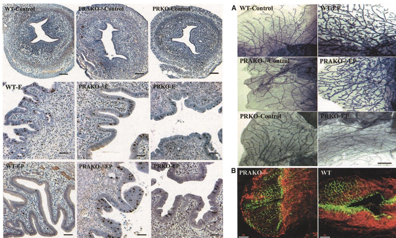
Fig. 3 (left). Abnormal proliferative responses to E and P treatment in PRAKO -/- uteri. BrdU immunolabeling of uteri from ovariectomized WT, PRAKO -/- , and PRKO mice treated with sesame oil (Control), E, or E plus P (EP). Bars, 200 \mu m (controls) and 50 \mu m (hormone-treated). Fig. 4 (right). Independence of mammary gland alveologenesis and tertiary ductal side branching from PR-A. (A) Thoracic
