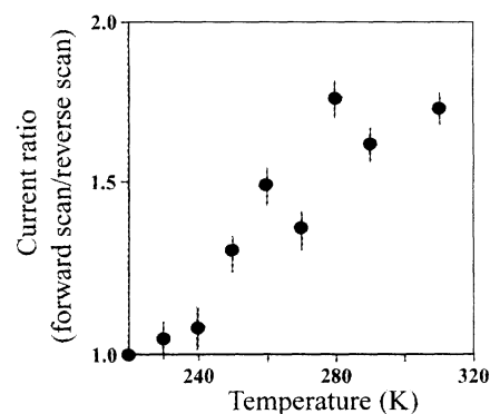
Fig. 3. Plotting the negative bias peak in the hysteresis ratio versus temperature represents the temperature dependence of the molecular switch. Near 220 K, the switching of the device is quenched, indicating that the mechanism of the device operation has at least one thermally activated step. Error bars represent the noise in the I - V measurements.
