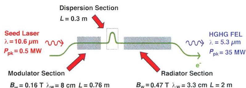
Fig. 2. Configuration for the HGHG FEL experiment as carried out at the Accelerator Test Facility at Brookhaven National Laboratory. The 40-MeV electron beam had a current of 120 A (0.8 nC in 6 ps) with a normalized emittance of 5 mm-mrad. L , length; \lambda , wavelength; P_{\text{pk}} , peak power; B_w , peak undulator magnetic field; \lambda_w , undulator period.
