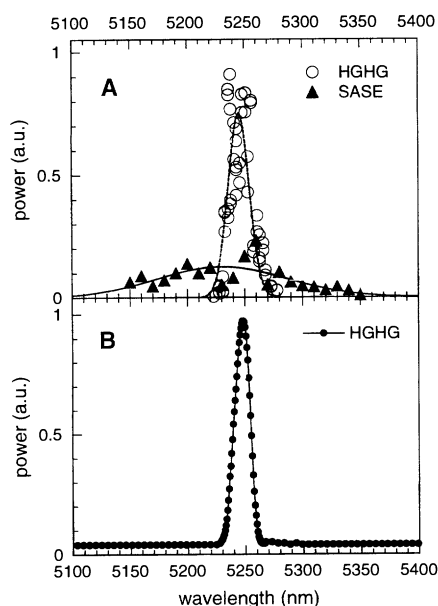
Fig. 3. Output spectrum. (A) Scanning multipulse measurements of the output power spectrum for HGHG and SASE, on the experimental apparatus illustrated in Fig. 2. The graph plots power (in arbitrary units) against wavelength (in nanometers). The HGHG FEL bandwidth is one-sixth the SASE bandwidth. The SASE data are multiplied by a factor of 10^6 to bring them onto the same scale as the HGHG results. The SASE amplifier could achieve the same power level as the HGHG FEL if the radiator undulator was made three times longer, but the SASE bandwidth would still be larger than that of the HGHG device. The solid line is a fit to the SASE spectral line, and the dashed line is a fit to the HGHG spectral line. (B) The HGHG single-shot spectrum as recorded by a thermal imaging camera placed at the exit plane of the spectrometer. The graph plots power (in arbitrary units) against wavelength (in nanometers). FWHM bandwidth is 15 nm.
