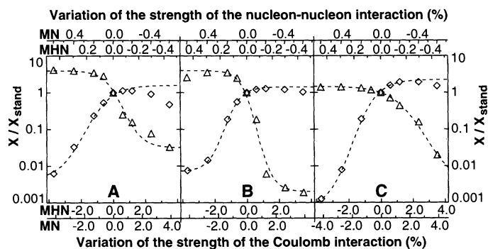
Fig. 1. The change of the C and O mass abundances through variations of the strengths of the strong and Coulomb interactions. The C mass abundance, X_C ( \Delta ), and the O mass abundance, X_O ( \diamond ), are shown in (A), (B), and (C) for stars with masses 20, 5, and 1.3M_{\odot} , respectively, in units of the standard values, X_{\text{stand}} . The variations of the strength of the strong and Coulomb interaction are given in the upper and lower scales for the two effective N-N forces MHN and MN. Dashed curves are drawn to show the trends.
