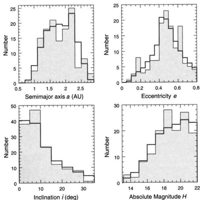
Fig. 2. A comparison between the 138 Spacewatch NEAs (shaded histogram) and n(a, e, i, H) (dark solid line), our best fit of the observed NEA probability distribution assuming \alpha_{3:1} , \alpha_{\text{IMC}} , \alpha_{v_6} = 0.36, 0.29, 0.35 , respectively, and \gamma = 0.35 . The parameters are linked to the NEA target region ( 0.5 \text{ AU} < a < 2.8 \text{ AU} ; e < 0.8 , i < 35^\circ ; H < 22 ). Our four-dimensional ( a, e, i, H ) distribution has been collapsed into one dimension for this comparison.
