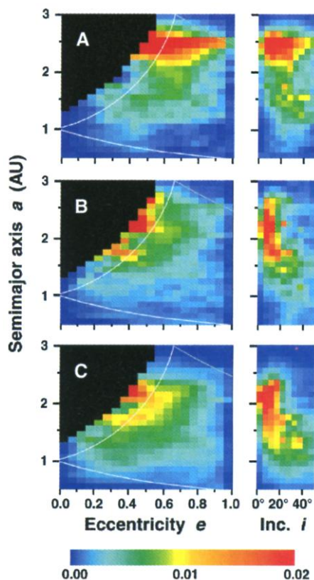
Fig. 1. A representation of the probability distributions of residence time [ R_{\text{IS}}(a, e, i) ] for NEAs evolving out of our three ISs: (A) 3:1 mean-motion resonance with Jupiter, (B) the IMC region, and (C) \nu_6 secular resonance. The sum of the ( a, e, i ) bins in the NEA target region ( 0.5 \text{ AU} < a < 2.8 \text{ AU} ; e < 0.8 ; i < 35^\circ ) has been normalized to 1.0. To display as much of the ( a, e, i ) distribution as possible in two dimensions, we summed the i bins before plotting R_{\text{IS}}(a, e) , whereas the e bins were summed before plotting R_{\text{IS}}(a, i) . The color scale depicts the expected density of NEAs in a scenario of steady-state replenishment from the IS regions. Red colors indicate where NEAs are statistically most likely to spend their time. Bins whose centers have perihelia q > 1.3 \text{ AU} are not used and are colored black. The white curved lines represent the values needed for an Earth-crossing orbit. The gray curve in the upper right indicates where objects cross the orbit of Jupiter.
