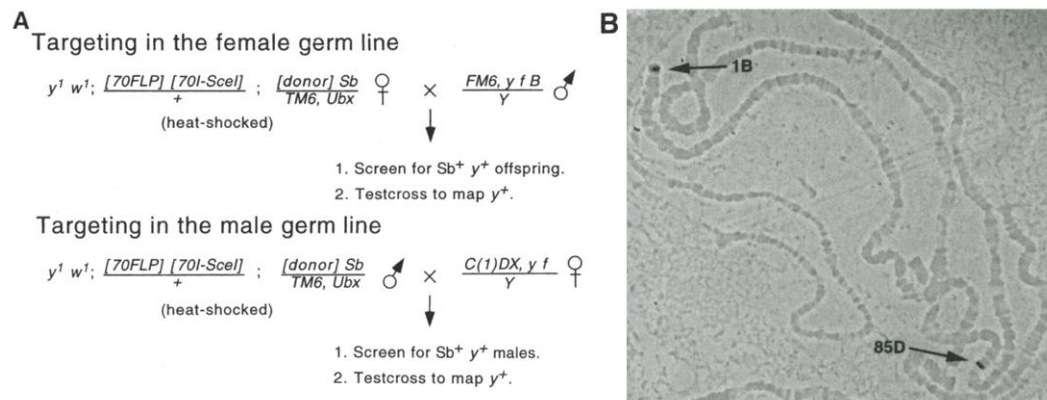
Fig. 3. Targeting the y gene. (A) Crossing schemes for yellow rescue (28). (B) Cytological localization of a targeted insertion. The cytological positions of \beta 2t hybridization are indicated on the chromosomes of this y'/y^+ class III female.
