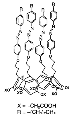
Fig. 1. Macrocyclic amphiphile tethering photochromic azobenzene units (CRA-CM).
