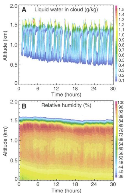
Fig. 2. Evolution of horizontal averages of (A) liquid water mixing ratio in cloud (grid cells with >0.05\text{ g/kg} liquid water) and (B) relative humidity in a baseline simulation. The profiles are output every 5 min.
