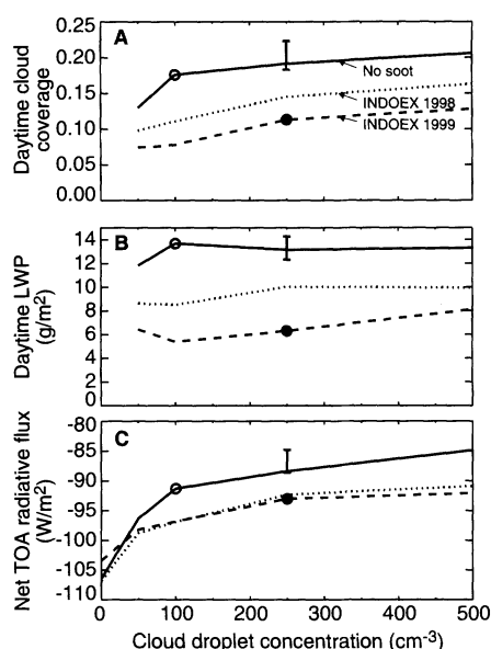
Fig. 5. Domain averages of (A) daytime fractional cloud coverage (as in Fig. 4, but averaged between 8 and 16 hours, during which 90% of solar energy is incident), (B) daytime liquid water path (as in Fig. 4), and (C) diurnal-average net radiative flux (in \text{W/m}^2 ) at the TOA. Diurnal averages are computed by averaging between 6 and 30 hours, thereby skipping over the first 6 hours of model spin-up. The net radiative fluxes for cloudless conditions are shown at a droplet concentration of zero. Variations with droplet concentrations (in \text{cm}^{-3} ) are shown for simulations in which the haze is nonabsorbing (solid line labeled "No soot"), and for the idealized 1998 and 1999 INDOEX hazes. The solid lines are drawn through the median values of the baseline ensemble; the error bars represent the ranges of ensemble values. Illustrative unpolluted and polluted conditions are shown as open and solid circles, respectively.
