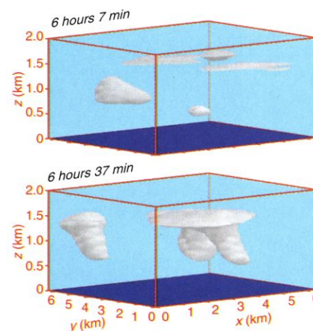
Fig. 3. Snapshots of the model domain taken during the early (6 hours 7 min) and mature (6 hours 37 min) growth stages of a convective episode. Plotted is the isosurface of 0.05\text{ g/kg} liquid water mixing ratio. Note that the vertical scale ( 2\text{ km} ) is stretched relative to the horizontal ( 6.4\text{ km} by 6.4\text{ km} ). Fractional cloud coverage [defined as in (13) by the fraction of columns with optical depth > 2.5 ] is 0.1 at 6 hours 7 min and 0.3 at 6 hours 37 min.
