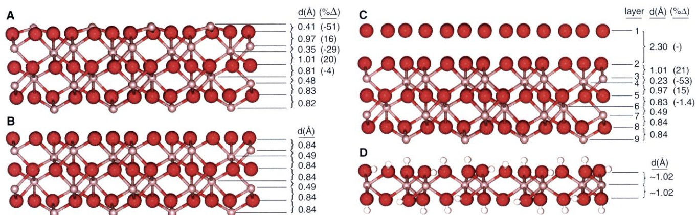
Fig. 2. (A to C) Atomic layering sequence and layer spacings ( d ) along the [0001] direction is shown for various terminations of the \alpha - \text{Al}_2\text{O}_3 surface. Red, silver, and gray spheres indicate O, Al, and H atoms, respectively. (A) Single Al-terminated surface model from Guenard et al. (17, 29). (B) Ideal (unrelaxed) oxygen-terminated surface. (C) Best-fit
