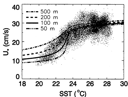
Fig. 3. A scatter plot of the weekly averaged values of U_* versus SST shown in Fig. 2. The spatial resolution of each value is 50 km. The four curves show the U_* -versus-SST relation given by a boundary layer model (26) having a thickness of 50 to 500 m. The air temperature and wind speed at the top of the boundary layer are assumed to be 24°C and 9 m/s, respectively.
