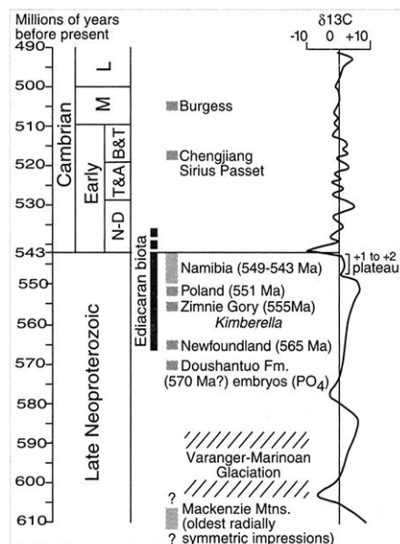
Fig. 1. Time scale showing temporal distribution of dated Ediacaran assemblages and several well-known Cambrian fossil assemblages (gray squares) and glaciations and carbon-isotopic curve. The ^{13}\text{C} isotopic curve is adopted from Knoll and Carroll (35). Phosphatized embryos that are similar to modern arthropods in the Doushantuo Formation of China are commonly cited as dated to 570 Ma (31, 36); however, there are no precise chronological constraints on this speculation of their age. Regional Siberian stage names are as follows: N-D, Nemakit-Daldynian; T&A, Tommotian and Atabanian; and B&T, Botomian and Toyonian; M, Middle; L, Late.
