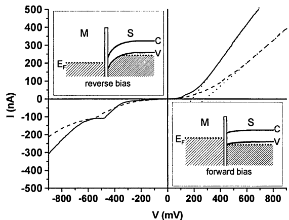
Fig. 3. Two-terminal I - V characteristics of two metallic SWNT-semiconducting SWNT junctions at a temperature of 50 K (solid and dashed lines). Bias was applied to the semiconducting SWNT. The dotted lines are linear fits to the forward bias data. The schematic energy level diagrams for the reverse bias (upper left inset) and forward bias (lower right inset) are shown.
