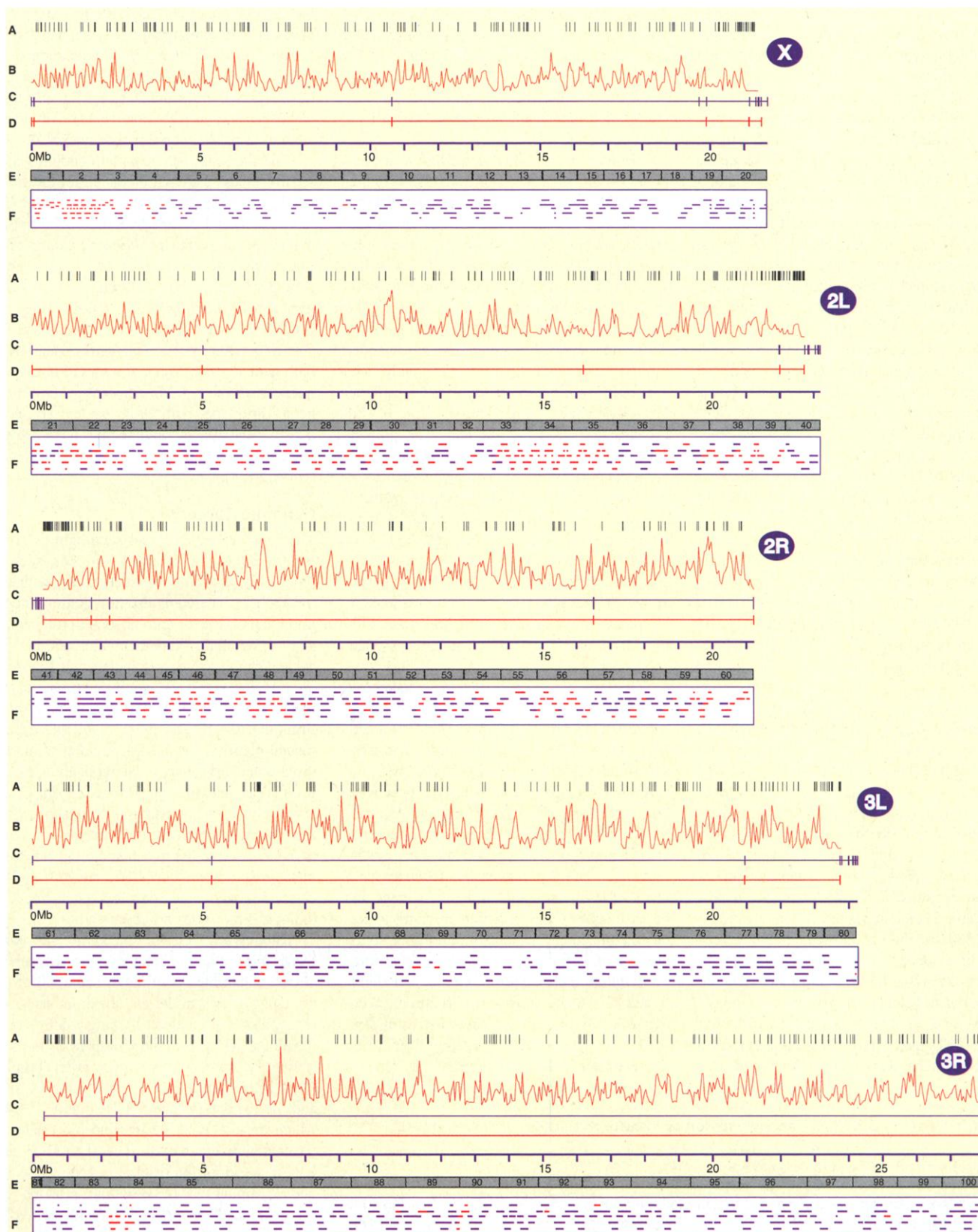
Fig. 3. Assembly status of the Drosophila genome. Each chromosome arm is depicted with information on content and assembly status: (A) transposable elements, (B) gene density, (C) scaffolds from the joint assembly, (D) scaffolds from the WGS-only assembly, (E) polytene chromosome divisions, and (F) clone-based tiling path. Gene density is plotted in 50-kb windows; the scale is from 0 to 30 genes per 50 kb. Gaps between scaffolds are
