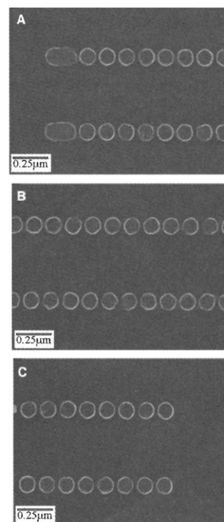
Fig. 1. Scanning electron micrographs of the left (A), center (B), and right (C) regions of two of the room temperature MQCA networks that we have fabricated.
