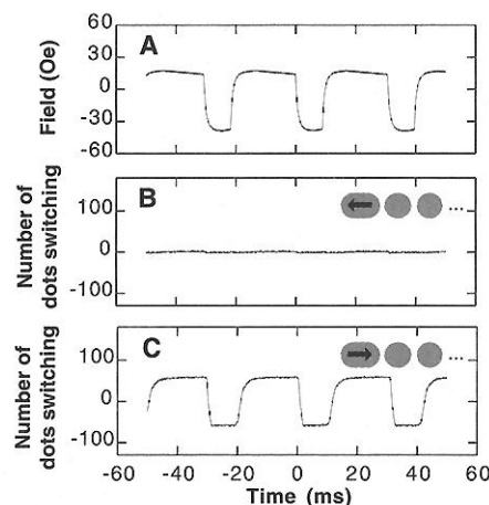
Fig. 2. Room temperature experimental results from the MQCA networks shown in Fig. 1: (A) The combined applied oscillating and bias fields; (B) the magneto-optical response of the MQCA networks for the case of the input dots set to 0 and (C) for the input dots set to 1, calibrated in number of dots switching within one network. The width of the edge transitions in (C) is not due to the temporal response of the MQCA networks but rather to a small distribution in switching fields, combined with the finite switching time of the applied oscillating field.
