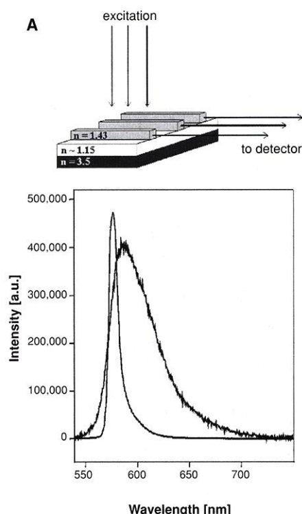
Fig. 5. (A) Emission spectra collected normal to the excitation beam along the waveguide axis at two different pump power densities ( 0.8 \text{ kW cm}^{-2} and 42 \text{ kW cm}^{-2} ). The low-power spectrum was multiplied to be clearly visible. a.u., arbitrary units. (B and C) Optical images of the axial output beams recorded with a CCD camera (B) below and (C) above the threshold power density. The width of each waveguide is 2.4 \mu\text{m} . The green background stems from the exciting laser beam.
