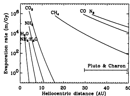
Fig. 5. Evaporation rates (in meters per billion years) of ices from the surface of an object in the outer solar system. The rates were calculated by assuming equilibrium between the temperature-dependent vapor pressure of the ice and the pressure of the escaping gas immediately above the surface of the object (21). AU, astronomical units.
