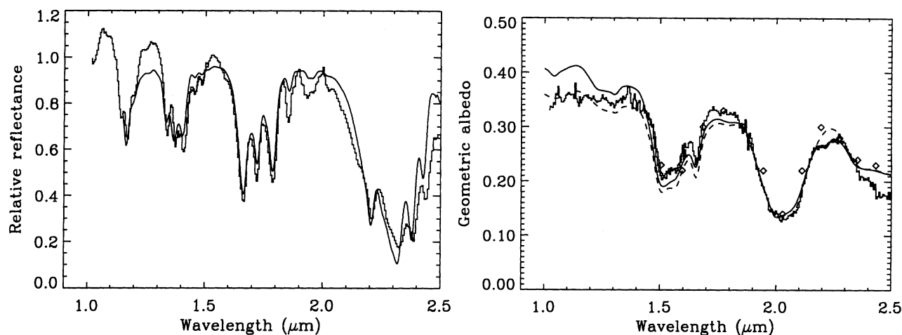
Fig. 2 (left). The near-infrared spectrum of Pluto. The histogrammed points give the data, scaled to a value of unity at a wavelength of 1.5 \mu\text{m} , and the smooth line is a reflectance spectrum of pure methane ice from Fink and Sill (7). The surface of Pluto is also known to contain \text{N}_2 and \text{CO} , but the weak spectral features due to these ices are not readily visible at this spectral resolution. Fig. 3 (right). The near-infrared
