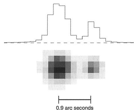
Fig. 1. Images of Pluto (left) and its satellite Charon (right) at the K band ( \sim 2 \mu\text{m} ). The objects are spaced by 0.90 arc seconds and are separated in the 0.30-arc second seeing. The histogram above the image gives a trace of the intensity through the center of the system, showing how little of the light from Pluto contaminates the spectrum of Charon.
