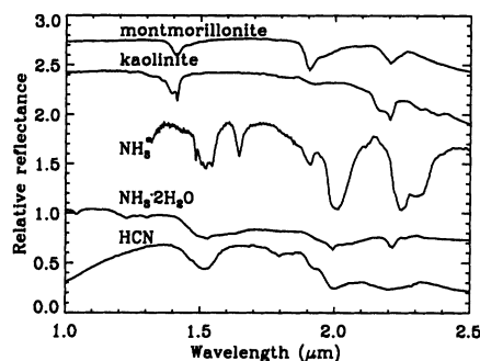
Fig. 4. Spectra of candidates for the 2.2- \mu\text{m} absorption seen on Charon (20). Montmorillonite and kaolinite are aluminosilicate clays.
