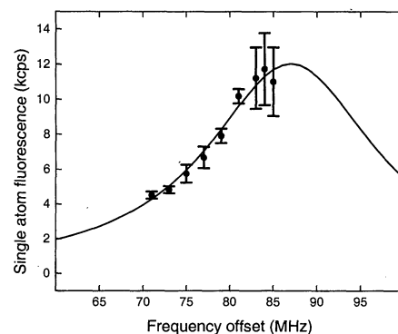
Fig. 3. Single-atom fluorescence versus laser frequency offset. Laser frequency offset indicates detuning from the reference line. Measured photon-count rates are fitted to a Lorentzian function, rates \propto [(f - f_r)^2 + (\gamma/2)^2]^{-1} . Here, f_r is the resonant transition frequency of ^{85}\text{Kr} , f is the laser frequency, and \gamma = \Gamma(1 + s)^{1/2} is the power-broadened linewidth. We fixed f_r = 87 MHz and \Gamma = 5.3 MHz according to previous spectroscopy measurements (27). The resulting saturation parameter s = 19 \pm 3 . Error bars represent change in fluorescence between different atoms. We attribute the cause of large fluctuations near resonance to the fact that the atom trajectory partially extends beyond the viewing region as the trap temperature increases near resonance. This effect was also observed on ^{83}\text{Kr} traps with a charge-coupled device camera.
