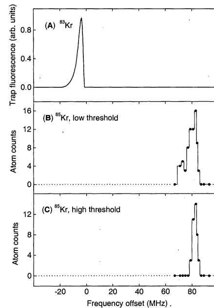
Fig. 4. (A) Fluorescence of trapped ^{83}\text{Kr} atoms versus laser frequency. Fluorescence was measured with a low-gain photodiode detector. (B and C) Number of ^{85}\text{Kr} atoms counted versus laser frequency. Each data point represents number of atoms counted in 20 min, with 10 min each for loading and counting. Fluorescence threshold, over which an atom is counted, was set at 3 kcps (B) and 10 kcps (C).
