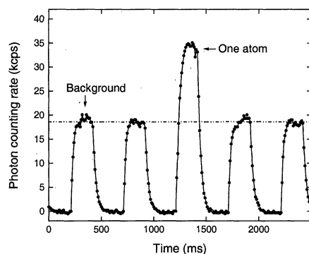
Fig. 2. Signal of a single trapped ^{85}\text{Kr} atom. During loading time, the photon-count rate was low because the counter was blocked for protection from overexposure.
