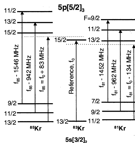
Fig. 1. Optimum laser frequencies for trapping ^{85}\text{Kr} and ^{81}\text{Kr} atoms. f_0 is the frequency of the reference transition in ^{83}\text{Kr} . f_{85} and f_{81} are frequencies of light for trapping ^{85}\text{Kr} and ^{81}\text{Kr} respectively. Note only hyperfine levels relevant to trapping are drawn.
