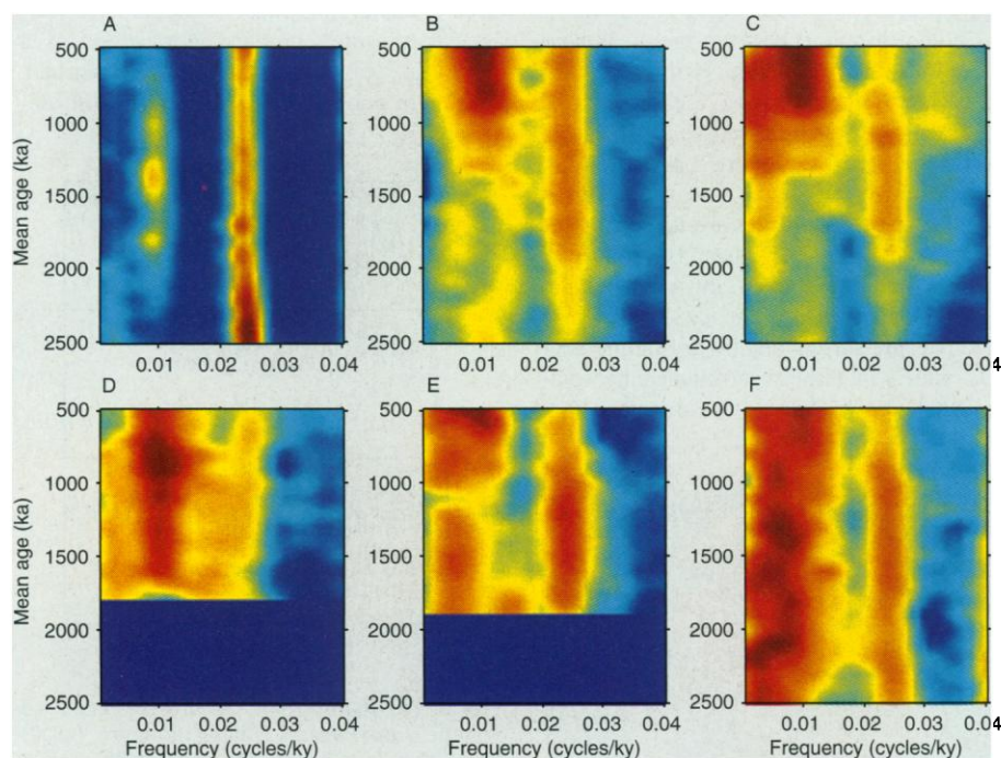
Fig. 7. Evolutive spectra (112) for (A) variations in eccentricity and tilt (101), (B) \delta^{18}\text{O} (per mil) from ODP Site 849 in the Pacific Ocean (2), (C) \delta^{13}\text{C} (per mil) from Deep Sea Drilling Project (DSDP) Site 607 in the North Atlantic (21), (D) the percent biogenic silica from Lake Baikal (65), (E) the grain size ratio of <2\ \mu\text{m} to >10\ \mu\text{m} from Chinese loess (67), and (F) the percent lithogenic detritus from ODP Site 722 in the northwest Arabian Sea (66). Variance is expressed as a logarithm for all figures except (A), which is plotted on a linear scale. Red colors are high values of variance, lighter blues are low values, and dark blue areas on (D) and (E) are no data. These data suggest that growth and decay of ice sheets influenced the rate of formation of NADW (C) (21), temperatures and aridity of northern and eastern Africa (64) and Asia (D, E) (65–67), the East Asian winter monsoon (67), and the Asian summer monsoon (66). Before the onset of Northern Hemisphere glaciation ~2.54 Ma, Asian temperature and hydrology and low-latitude monsoonal climate were responding to regional precessional and obliquity forcing. After 2.5 Ma, changes in Asian and African climate became largely in phase with or lagged changes in the ice sheets (64–67), indicating that they are now driven largely by the ice sheets through their influence on the atmosphere. A substantial increase in 100-ky variance in these proxies after the middle Pleistocene transition in association with the onset of large 100-ky ice-sheet cycles further identifies these ice sheet–climate relations. [Figure courtesy of N. G. Pisias.]
