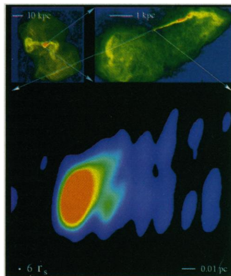
Jet propulsion. New VLBA image of the core region of M87. Earlier radio images of the galaxy at larger scales are shown above.
