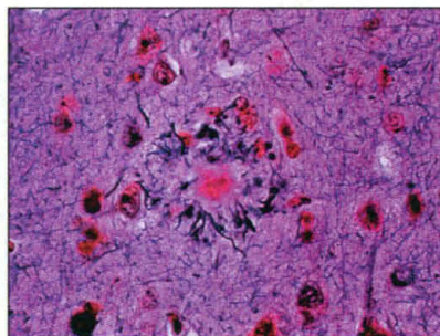
Plaque production. By cleaving the precursor protein (APP), BACE and \gamma -secretase release \beta -amyloid ( A\beta ), which forms plaques (right).
