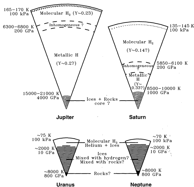
Fig. 1. Schematic representation of the interiors of Jupiter, Saturn, Uranus, and Neptune. The hashed region indicates a possible radiative zone [in Jupiter, it corresponds to P \sim 0.15 to 0.6 GPa, T \sim 1450 to 1900 K, and R \sim 0.990 to 0.984 R_J ; in Saturn, it is located around P \sim 0.5 GPa, T \sim 1700 K, and R \sim 0.965 R_S , but it is probably very marginal (23)]. The range of temperatures for Jupiter and Saturn is for models neglecting the presence of the inhomogeneous region. Helium mass mixing ratios Y are indicated. In the case of Saturn, it is assumed that Y/(X + Y) = 0.16 in the molecular region. The size of the central rock and ice cores of Jupiter and Saturn is very uncertain (see text). Two representative models of Uranus and Neptune are shown, but their actual interior structure may be significantly different (34). The figure is adapted and updated from (19).
