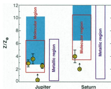
Fig. 2. Constraints on the mass mixing ratio of heavy elements, in solar units [assuming the mass mixing ratio of heavy elements in the sun ( Z_\odot ) = 0.0192 (58)] of the molecular (red rectangles) and metallic (purple rectangles) regions of Jupiter and Saturn. The helium mixing ratios used for the calculation are the Galileo value for Jupiter (13) and Y/(Y + X) = 0.16 \pm 0.05 for Saturn (see text). The enrichments in the molecular regions that would have been found with the old Voyager values (13, 15) are indicated by blue areas. When available, the observed abundances of C, N, O, and S are indicated. The maximum value for the heavy element enrichment of Saturn's metallic region is 20 Z_\odot .
