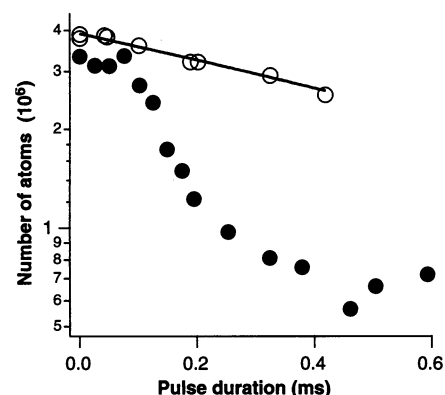
Fig. 2. The decay of atoms in the condensate at rest showed the normal exponential decay for parallel polarization (O) and faster superradiant decay for perpendicular polarization (●). The laser intensities (13 \text{mW}/\text{cm}^2 ) and oscillator strengths were equal in both cases.
