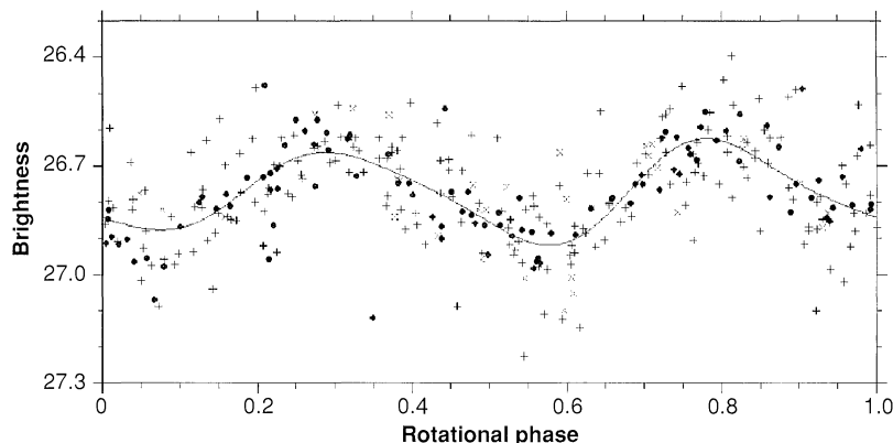
Fig. 2. Composite light-curve constructed for P = 10.7015 min from clear-filter photometry obtained at Ondřejov on June 2.0 ( \times ) and June 3.0 ( + ) and at Spacewatch on June 5.3 ( \bullet ). Brightness is in visual (V) magnitudes, scaled to correspond to geocentric and heliocentric distances of 1 AU and an Earth-asteroid-sun angle of 28.1^\circ . The rotation phase origin is at 1998 June 5.3045. The noise level of individual measurements, about 0.1 magnitude, reflects the asteroid's faintness and our short integration times (20 to 50 s). The light-curve data are represented well by a fourth-order Fourier series (solid curve).
