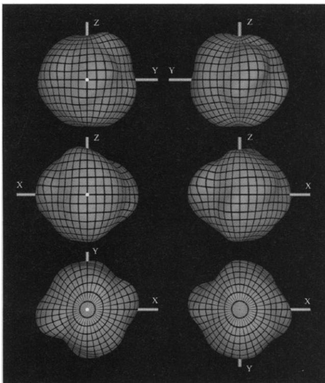
Fig. 3. Asteroid 1998 KY26's shape estimated from least-squares fitting of a 124-vertex polyhedral model to the echo spectra. The effective resolution of the model is 3 m. The model solution depends on the subradar latitude \delta , which is not known but probably was at least a few tens of degrees from the pole. This figure shows the solution for an equatorial view ( \delta = 0 ). The fractional topographic relief is fairly insensitive to \delta . The model's mean diameter is 26 m/cos \delta . Principal axes of inertia are labeled x, y, and z (the pole).
