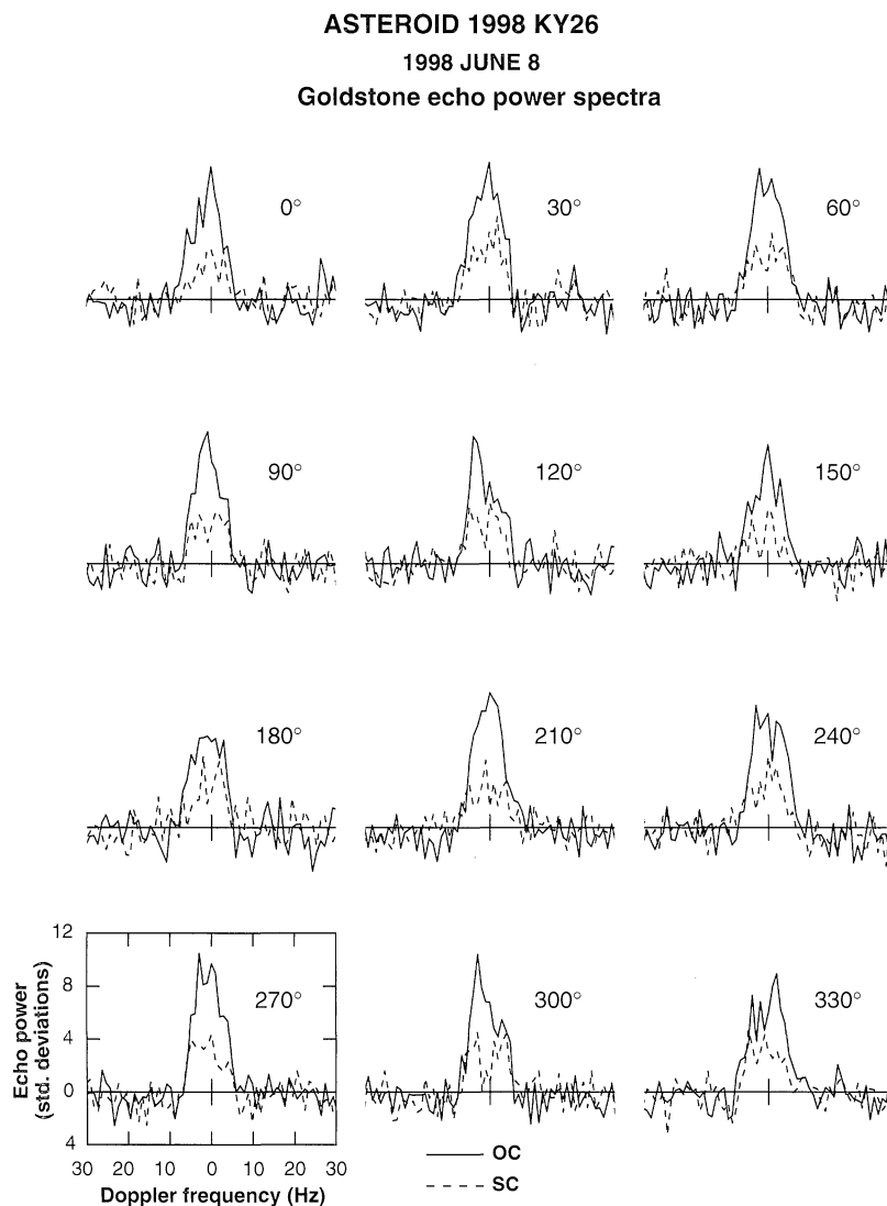
Fig. 1. Our strongest echo spectra from June 8, sorted into rotation-phase bins 30^\circ wide. Our analyses used 15^\circ bins. Each spectrum is a one-dimensional image equivalent to a scan of radar brightness measured through a slit parallel to the asteroid's projected apparent pole. The frequency resolution, 1 Hz, corresponds to a slit width of 1.8 \text{ m}/\cos \delta , with \delta the subradar latitude. The rotation phase origin is at 1998 June 8.2600.
