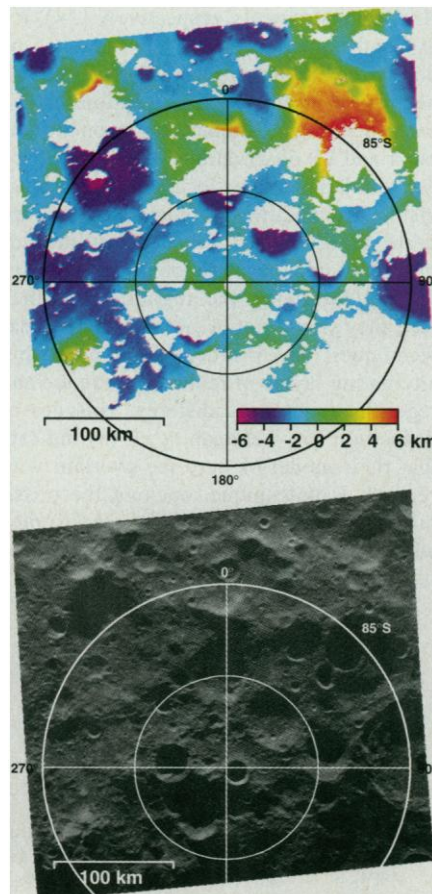
Fig. 2. Digital elevation model (top) and radar backscatter map (bottom) of the south polar region. Absolute elevations with respect to a sphere with a radius of 1738 km are shown. Maps are stereographic projections and use east longitudes.
