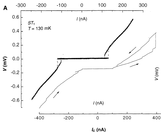
Fig. 3. (A) (Upper curve) V(I) characteristics for ST_1 , from which the critical current is deduced. (Lower curve) The same data on a wider current scale showing the existence of voltage steps for currents higher than i_c . (B)
