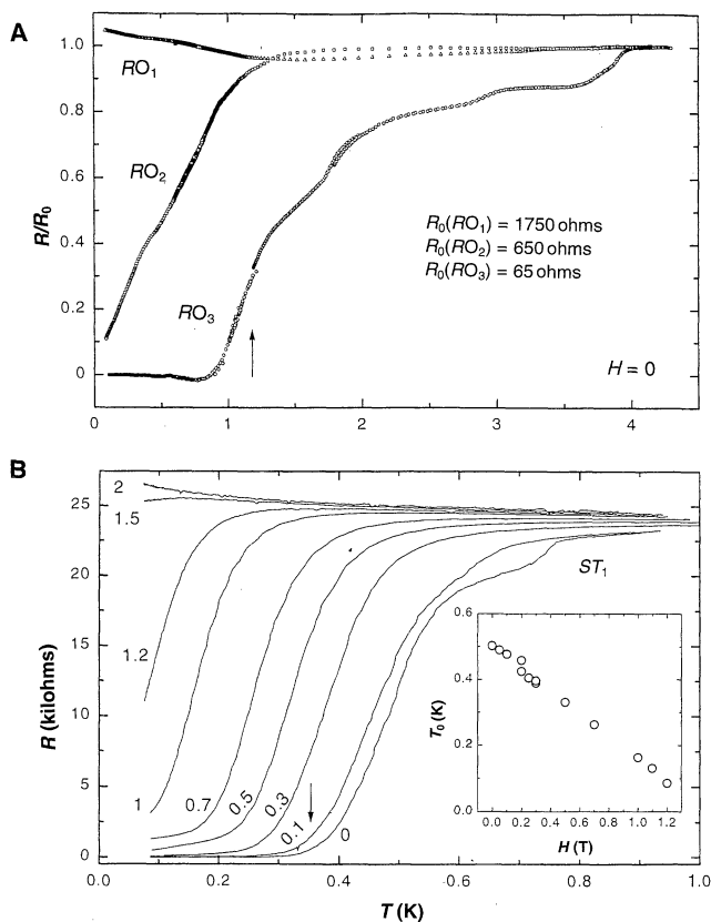
Fig. 2. (A) Temperature dependence of the resistance of ropes RO_1 , RO_2 , and RO_3 mounted on Au/Re contacts measured for zero magnetic field. The arrow indicates the transition of the Au/Re bilayer. The sample RO_3 becomes superconducting below 1 K, but the existence of resistance steps above the transition indicates that superconductivity may not be homogeneous. (B) Temperature dependence of the resistance of the single tube ST_1 mounted on Au/Ta measured for different values of the magnetic field perpendicular to the tube axis. (The labels on the curves correspond to the value of magnetic field in Tesla.) The arrow indicates the transition temperature of the contact in zero magnetic field. (Inset) Field dependence of the transition temperature [defined as the inflexion point of R(T) ].
