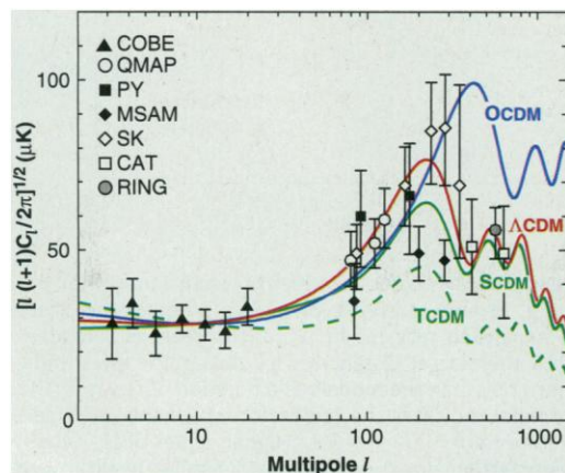
Fig. 6. The CMB temperature anisotropy is presented as a function of angular scale. The multipole l corresponds roughly to an angular scale of \pi/l radians. Flat models ( \Omega_m + \Omega_\Lambda = 1 ) produce an acoustic peak at l = 200 (about 1^\circ on the sky). Open models have a peak that is shifted to smaller scales (larger l values). (The height of the peak depends on additional parameters, including \Omega_m , \Omega_\Lambda , \Omega_b , H_0 , and tilt; here, we use the model values from Table 1.) The observational data points (with 1\sigma error bars) include the COBE measurements on large scales (small l values) and other published, multifrequency ground- and balloon-based observations [QMAP (86), PY (87), MSAM (88), SK (89), CAT (90), and RING (91)].
