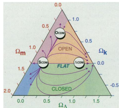
Fig. 7. The Cosmic Triangle: Past, Present, and Future. The past and future of the universe are represented by various trajectories in the cosmic triangle. The trajectories, which originate from near \Omega_m = 1 (an unstable equilibrium point matching the approximate condition of the universe during early structure formation), indicate the path traversed in the triangle plot as the universe evolves. For the current best fit \Lambda CDM model, the future represents a flat accelerating universe that expands forever, ultimately reaching \Omega_m \rightarrow 0 and \Omega_\Lambda \rightarrow 1 .
