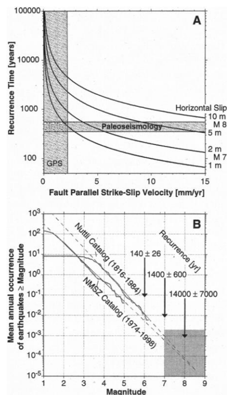
Fig. 4. (A) Relation between interseismic motion and the expected recurrence of large New Madrid earthquakes. For an assumed horizontal slip in 1811–1812 of 5 to 10 m, the geodetically observed interseismic motion of less than 2 mm/year implies recurrence times greater than 2500 years. Also shown are recurrence estimates from paleoseismic studies. The paleoseismic and geodetic data are jointly consistent with slip in 1811–1812 being about 1 m, corresponding to a magnitude 7 earthquake. (B) Earthquake frequency-magnitude data for the NMSZ. Both the recent and historic (1816 to 1984) data have slopes close to 1 and predict a recurrence interval exceeding 1000 years for magnitude 7 earthquakes and 10,000 years for magnitude 8 earthquakes. Estimates are shown with 2\sigma uncertainties.
