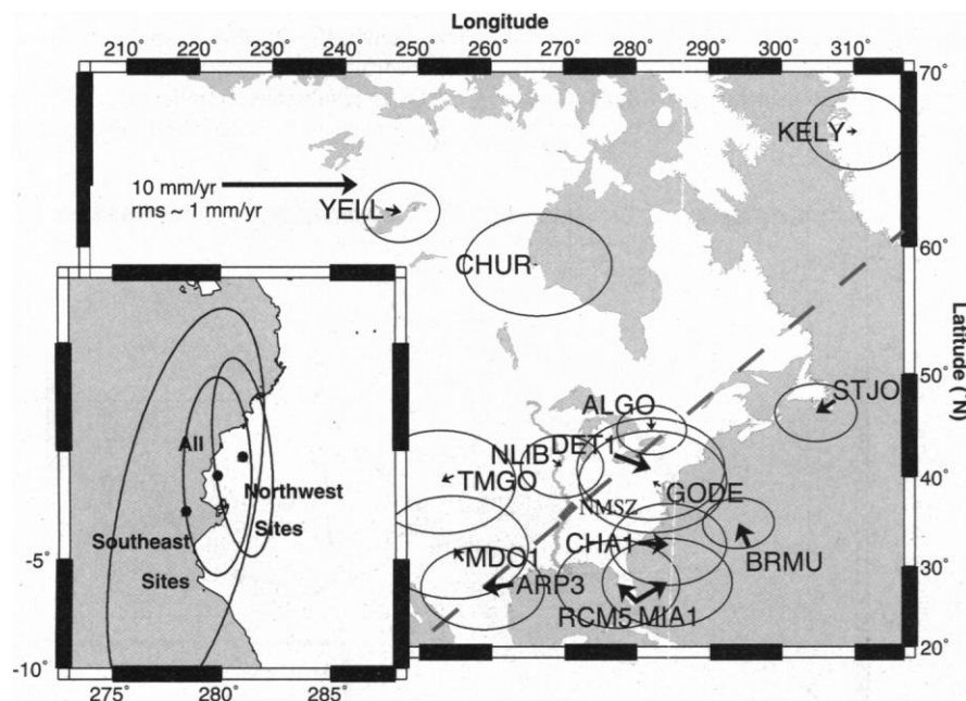
Fig. 3. Locations of continuously recording GPS sites used to estimate an Euler vector for the presumably stable portion of North America. For each, the misfit between the observed velocity and that predicted for a single plate is shown. (Inset) Euler poles for the eastern and western subsets of the sites (divided by dashed line in main panel) compared with that for the entire set. Because the poles for the east and west data overlap at 95% confidence, the platewide GPS data show no resolvable motion across the NMSZ.
