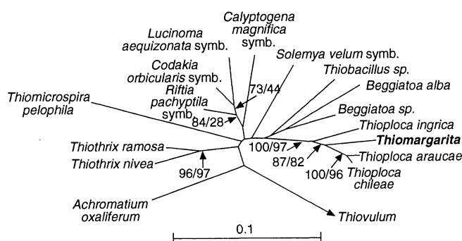
Fig. 3. Distance tree of Thiomargarita namibiensis and related sulfur-oxidizing bacteria of the gamma-proteobacterial subdivision. The distance tree is based on 16S rRNA position 358 to 802, which is the overlap of the partial 16S rDNA sequence of Thioploca araucae , T. chilae , and Thiomargarita . The tree was rooted with Thiovulum majus of the epsilon-proteobacterial subdivision as outgroup. Bootstrap values (200 runs) are given for nodes that have at least 70% support by distance (first) or parsimony bootstrap (second value). The bar corresponds to 0.1 Jukes-Cantor substitutions per nucleotide. The sequence has been deposited with GenBank (accession number AF129012).
